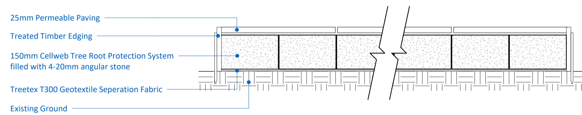
'No-Dig Construction' Driveway Section 1 : 10
