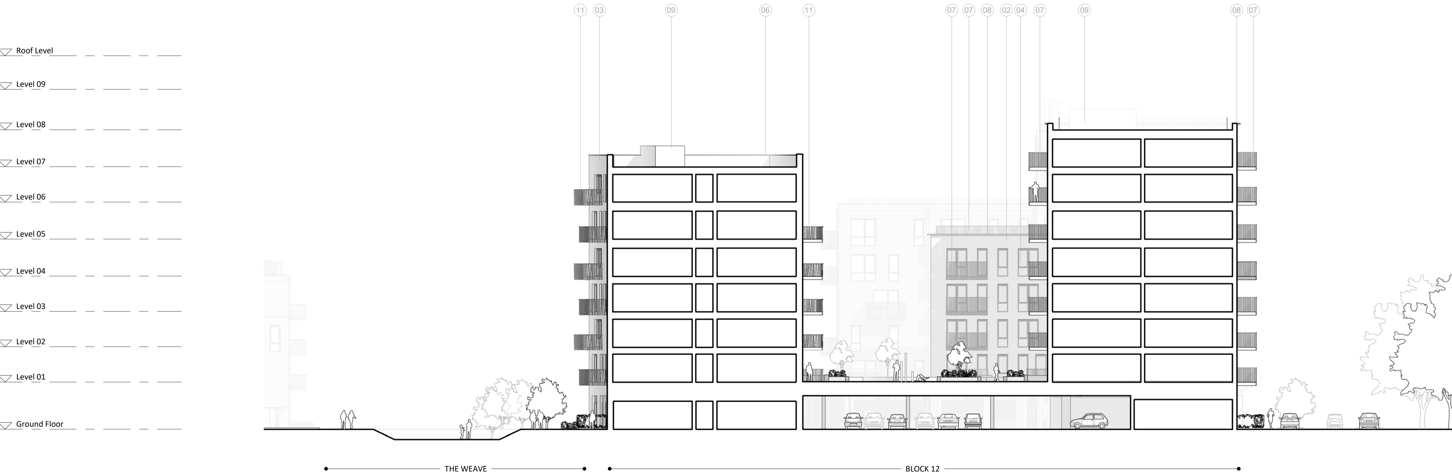
2 Podium Section - Looking South 1 : 200
