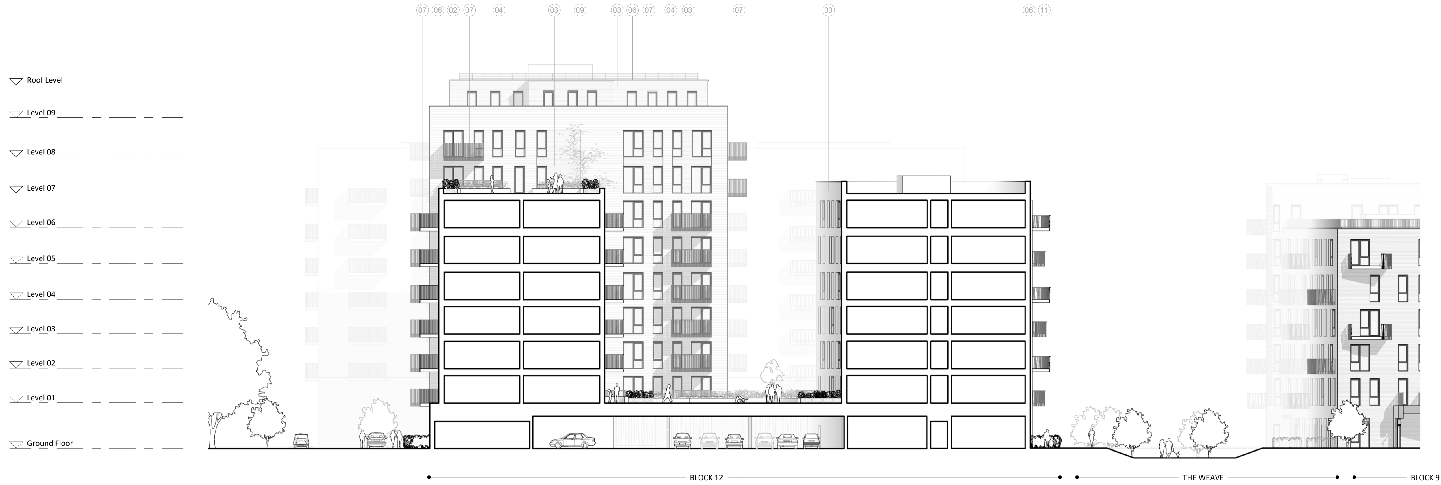
1 Podium Section Looking North 1 : 200
