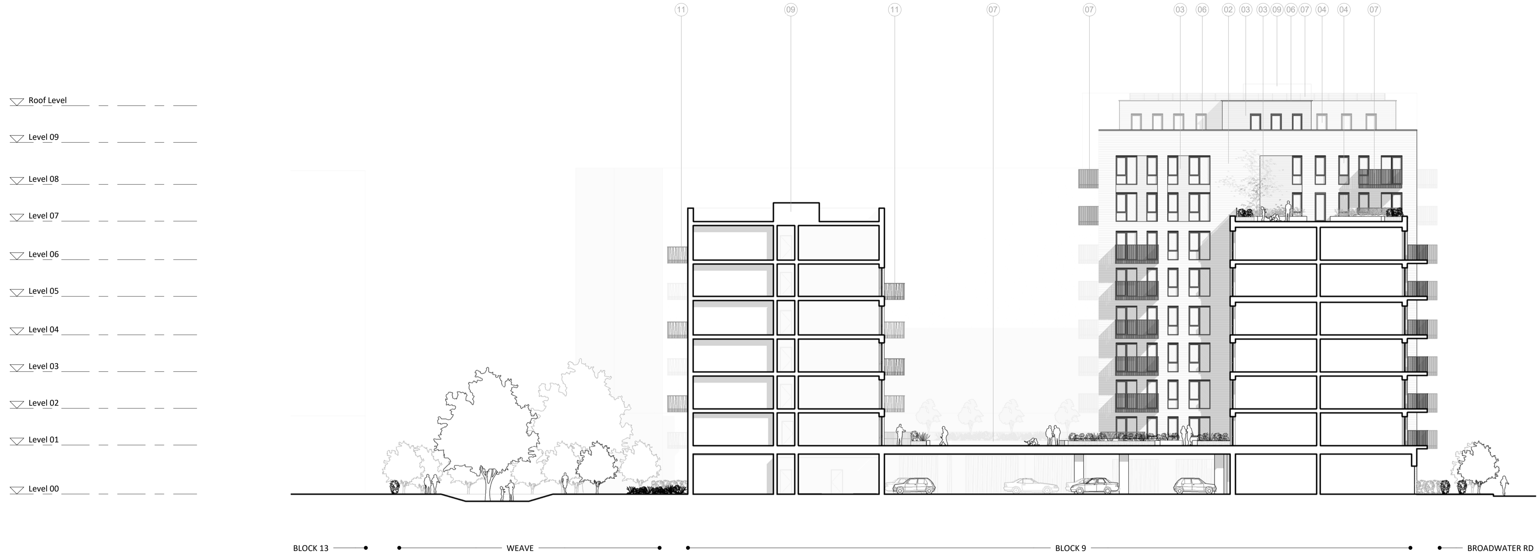
1 Podium Section Looking North 1 : 200
