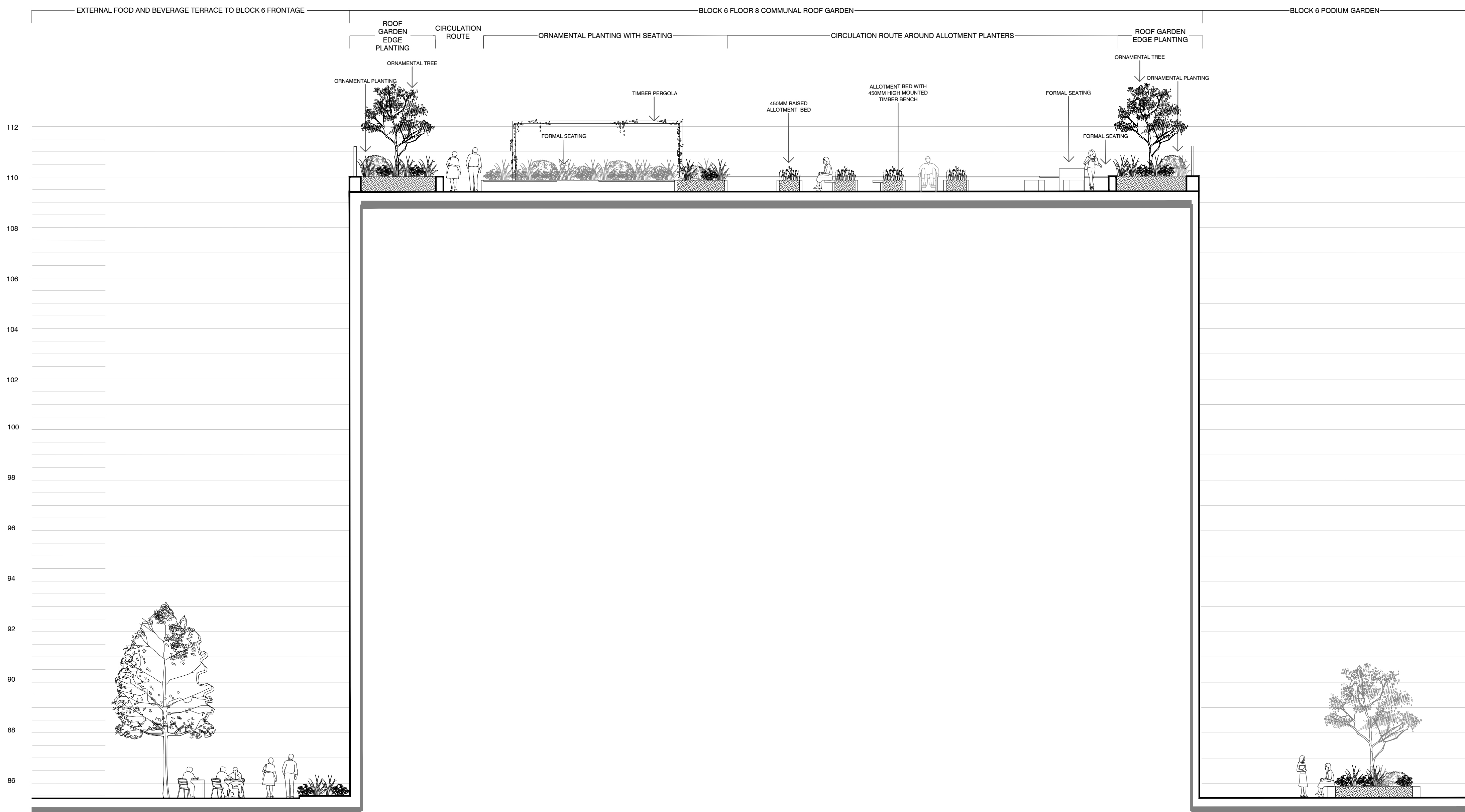
005 402 ROOF GARDEN - BLOCK 6 SECTION
