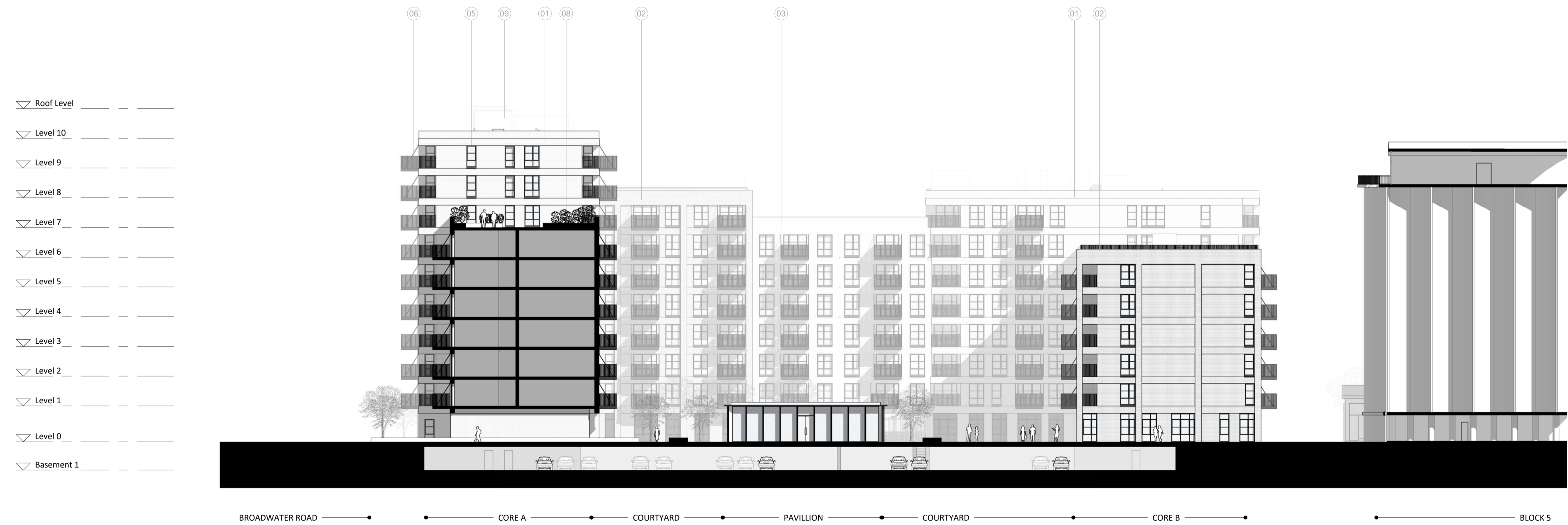
2 Block 7 - Section - Looking South 1 : 250
