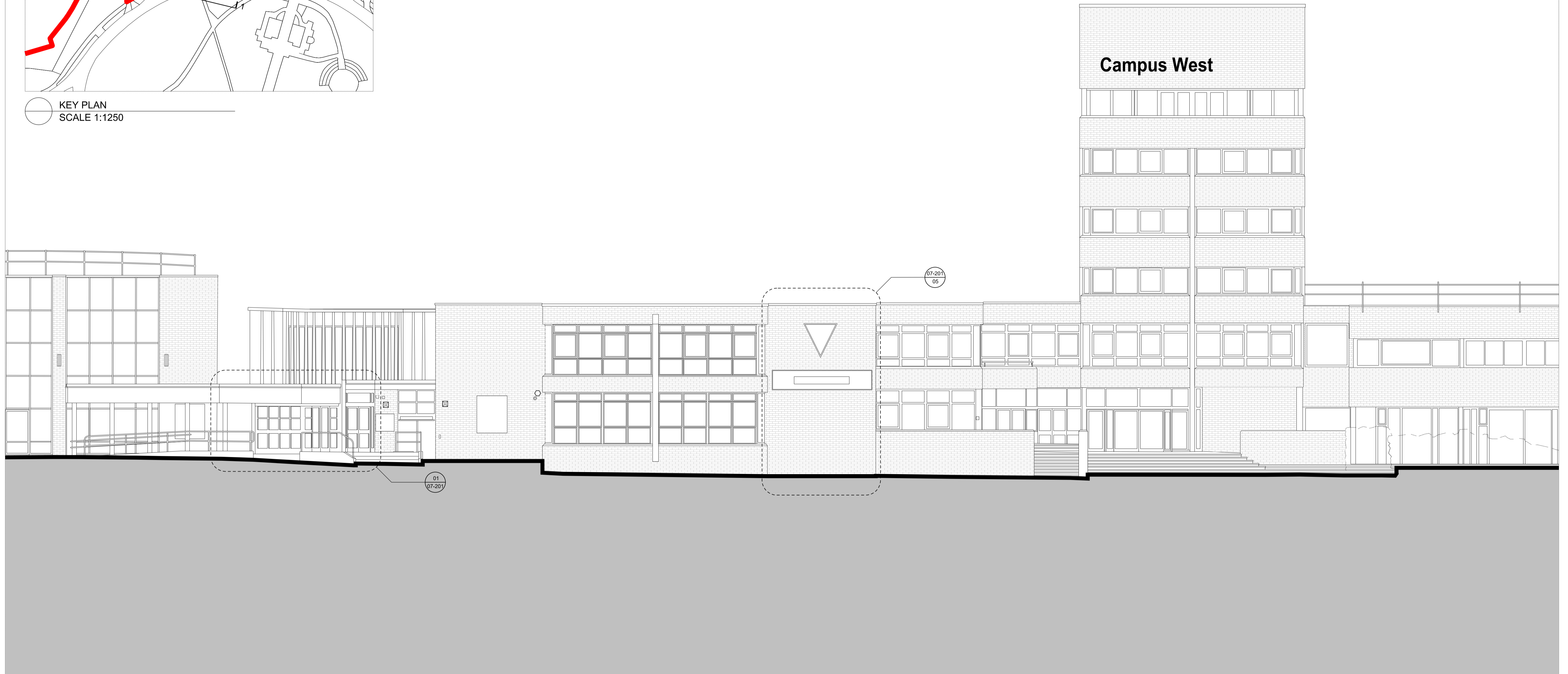
01 EXISTING SOUTHERN ELEVATION SCALE 1:100
