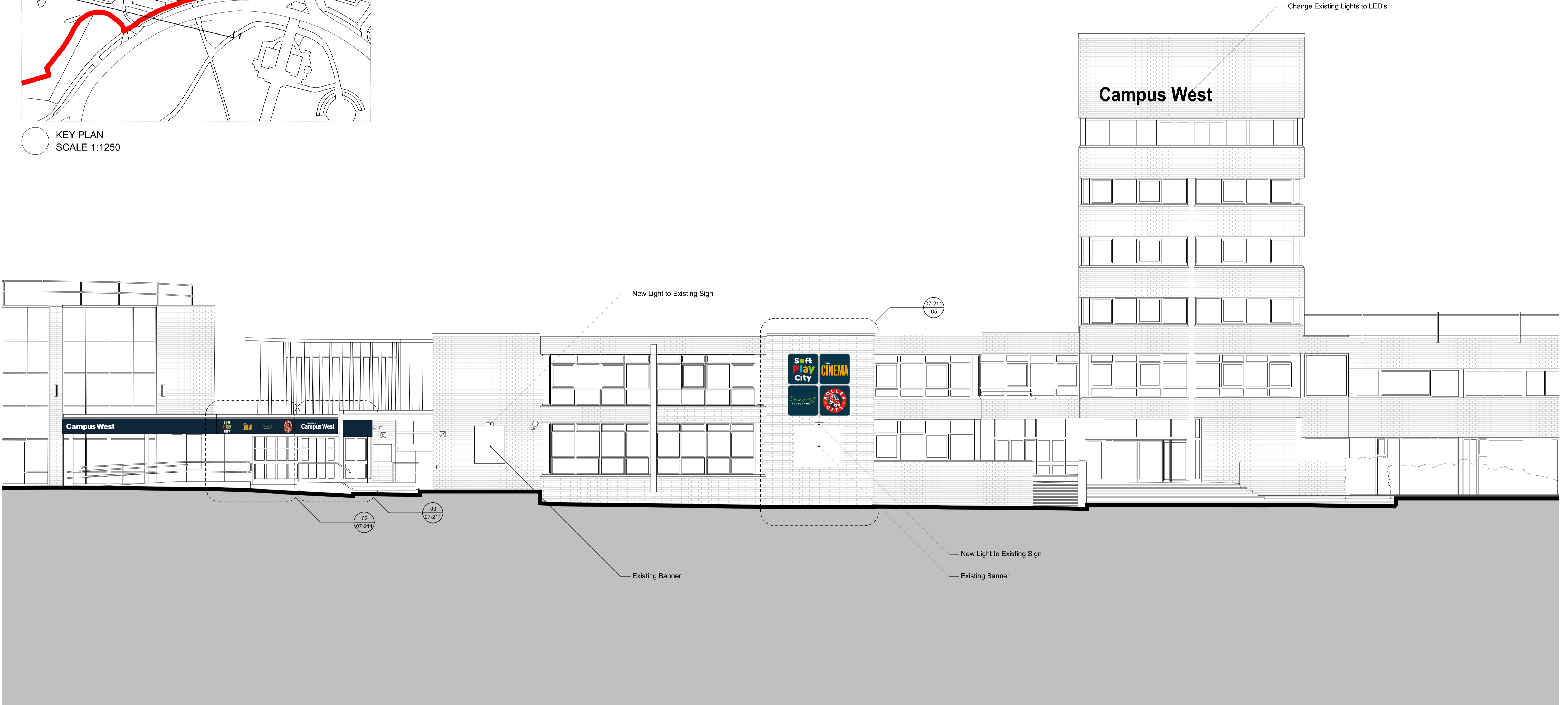
01 PROPOSED SOUTHERN ELEVATION SCALE 1:100
