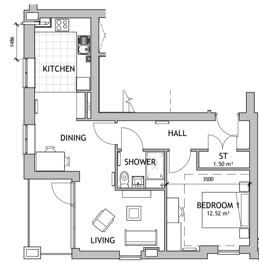
Flat M x 6 53.1m 2 1 : 100
