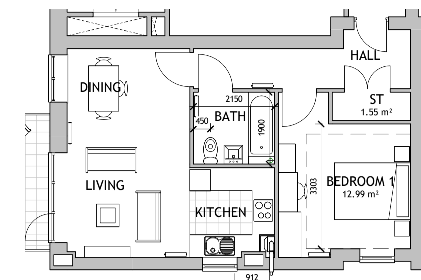
Flat L x 1 50.5m 2 1 : 100
