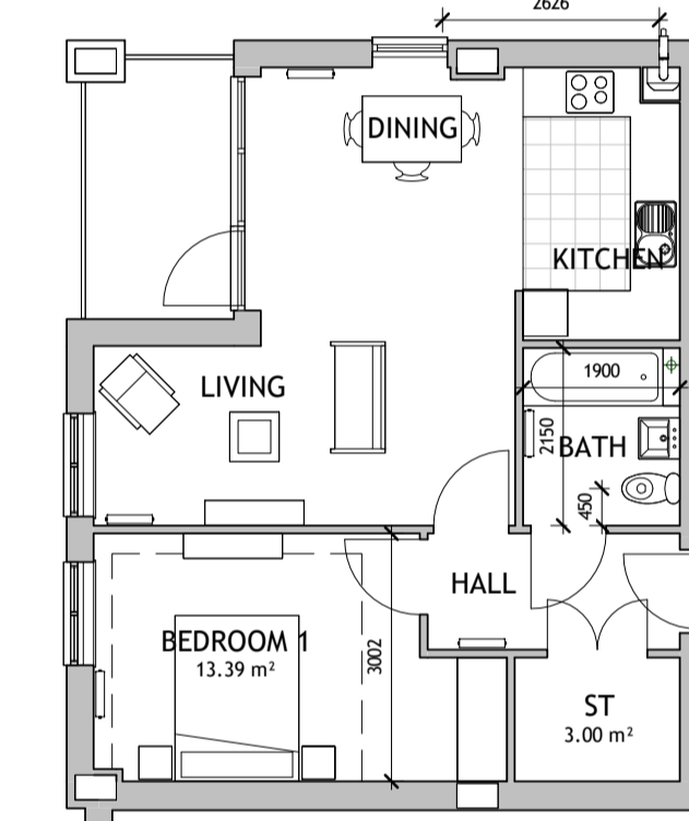
Flat O x 3 54.4m 2 1 : 100
