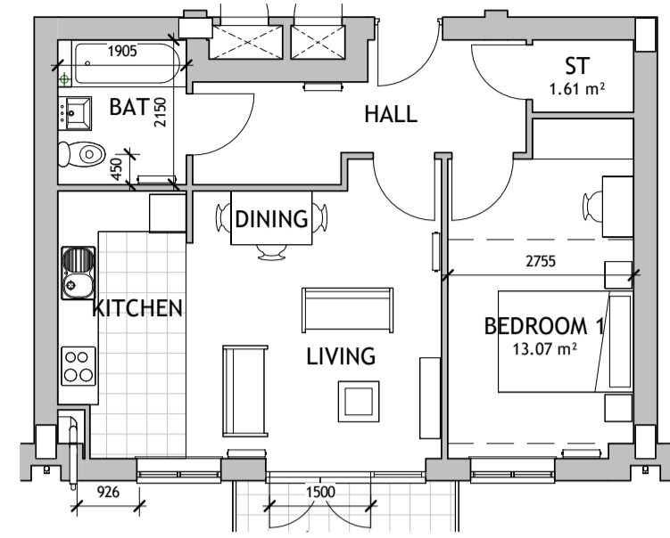
Flat J x 4 51.2m 2 1 : 100
