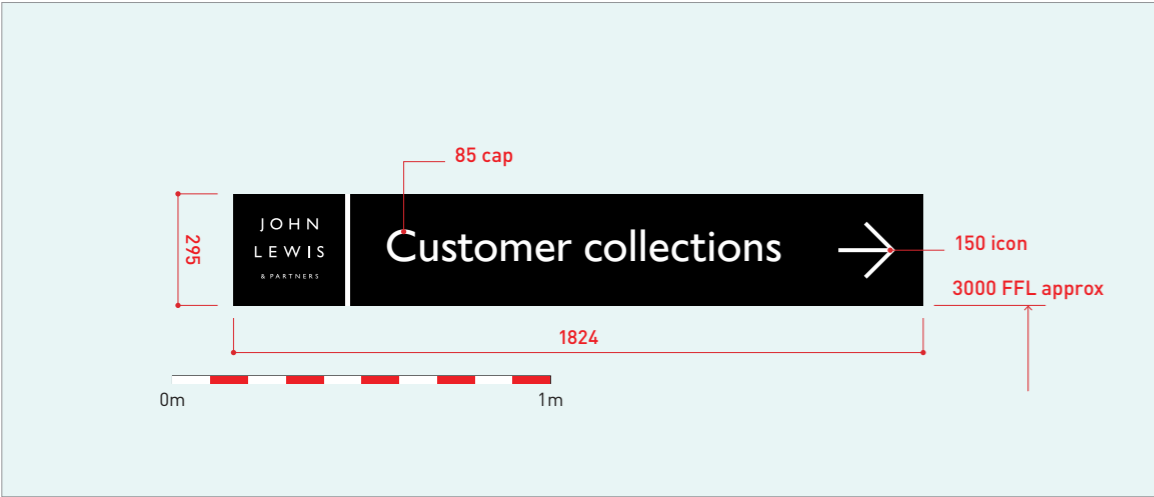
Sign detail (1:20 @ A3)
