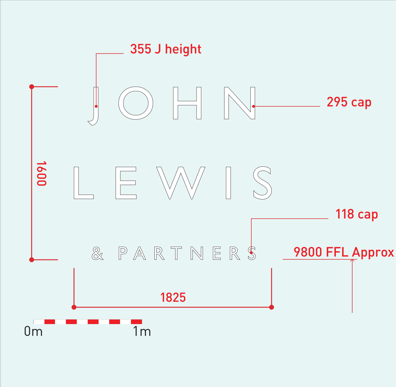
Sign detail (1:50 @ A3)
