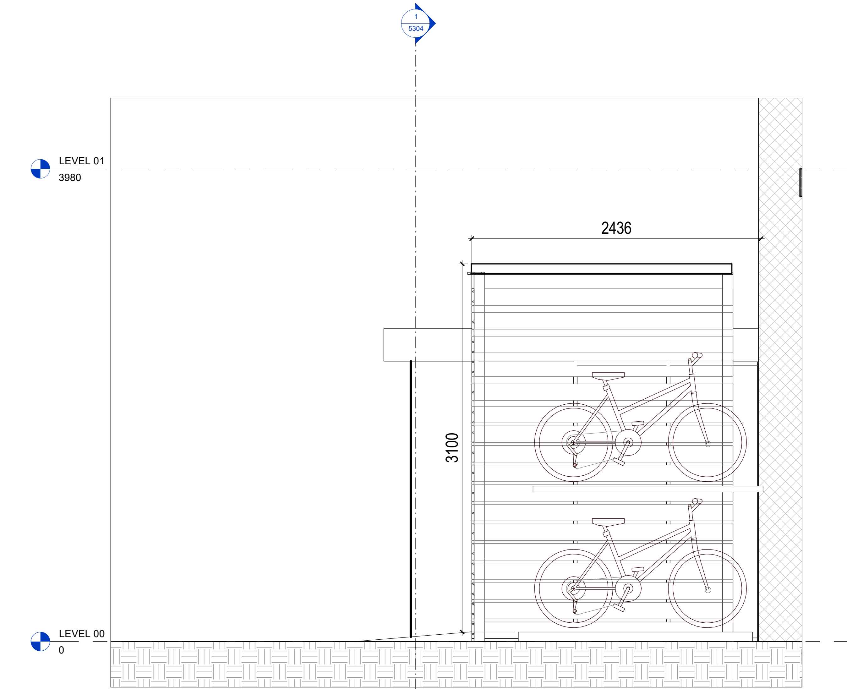
4 BIKE STORAGE SECTION 1:20
