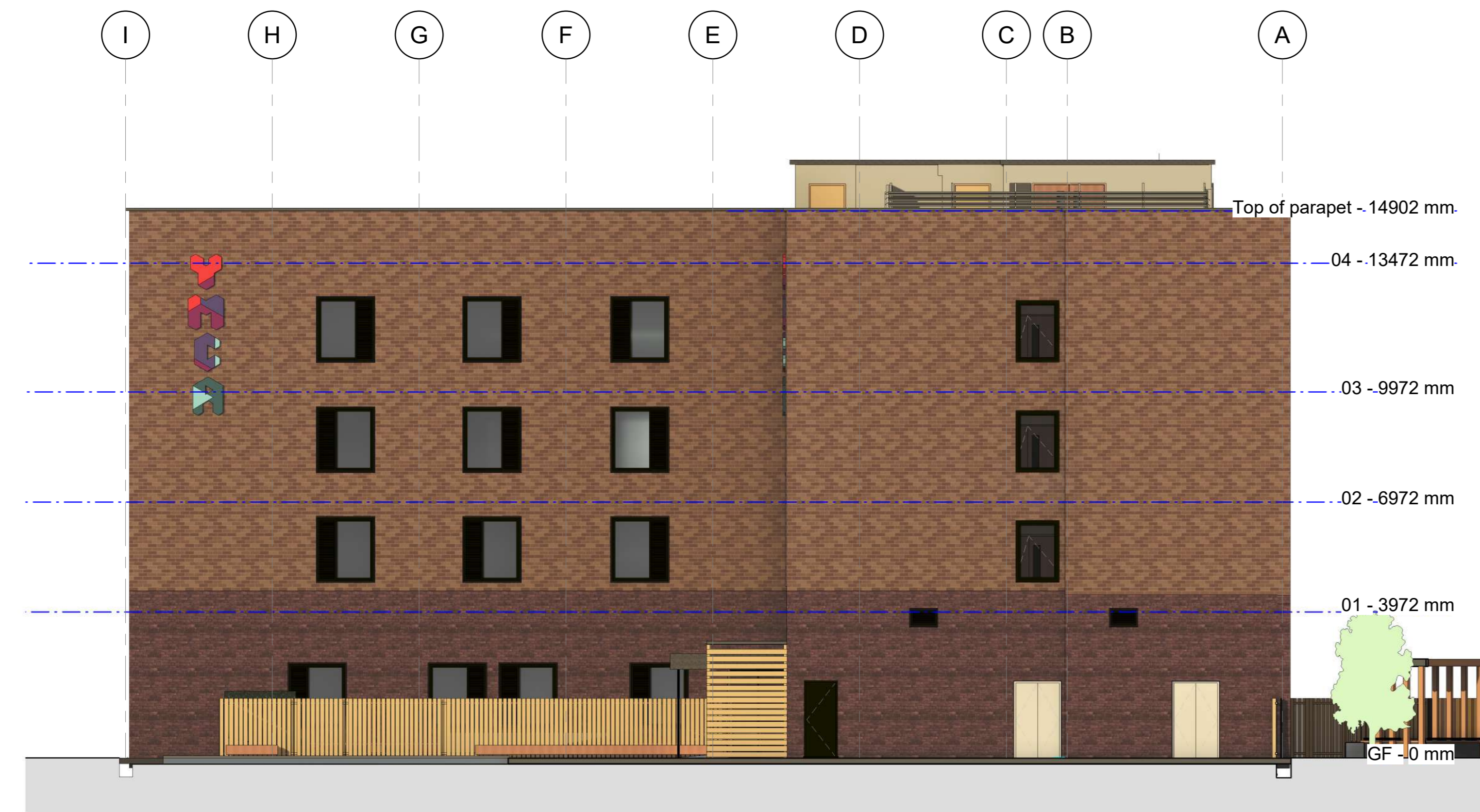
1 NORTH EAST ELEVATION 1 : 100
