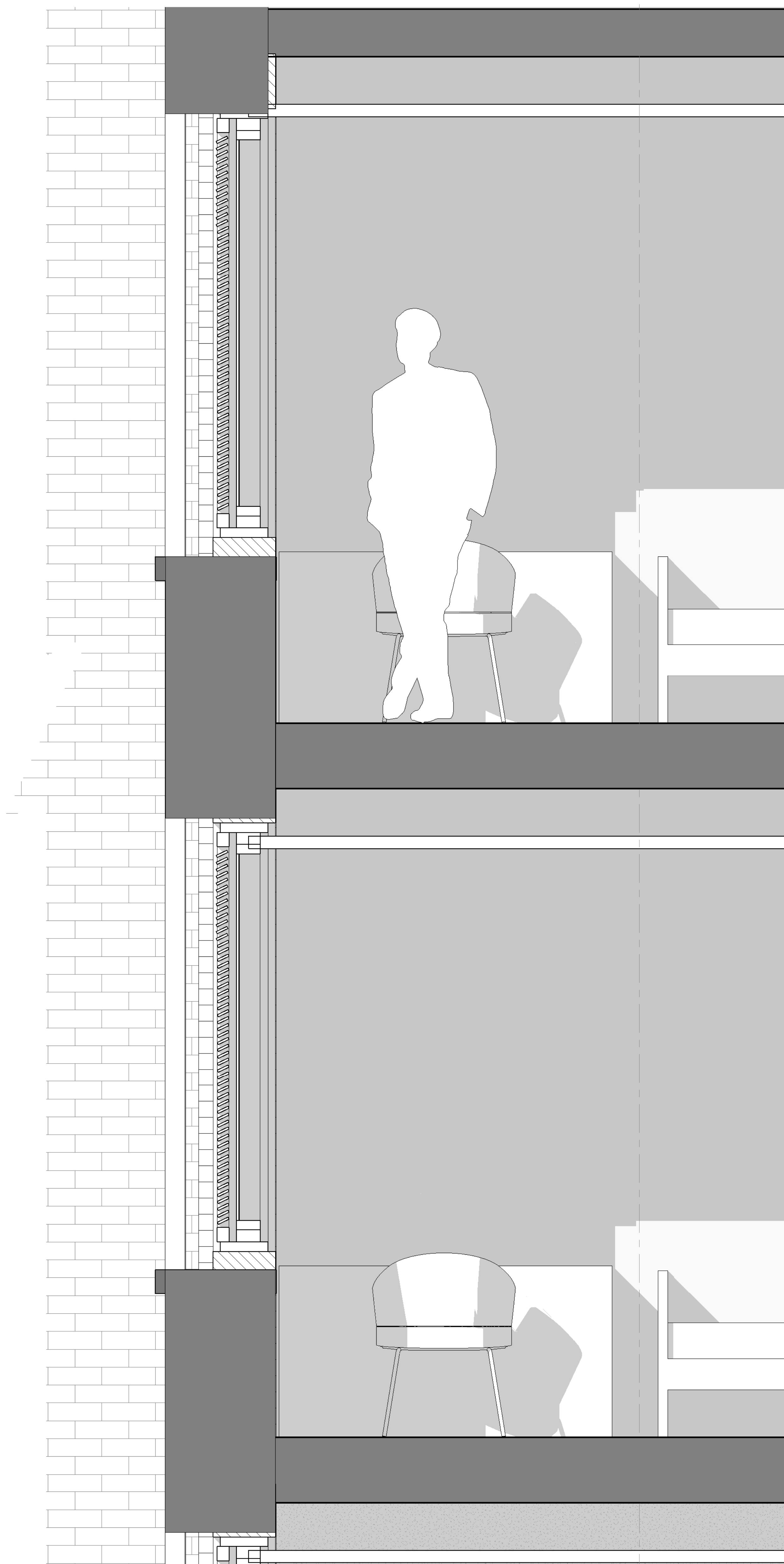
2 WINDOW DETAIL SECTION 1 : 10
