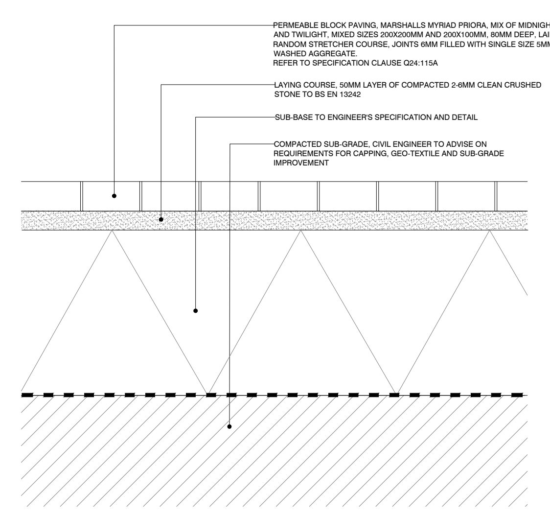
004 PERMEABLE BLOCK PAVING TO FOOTPATHS TYPE 2 SECTION SCALE - 1:10
