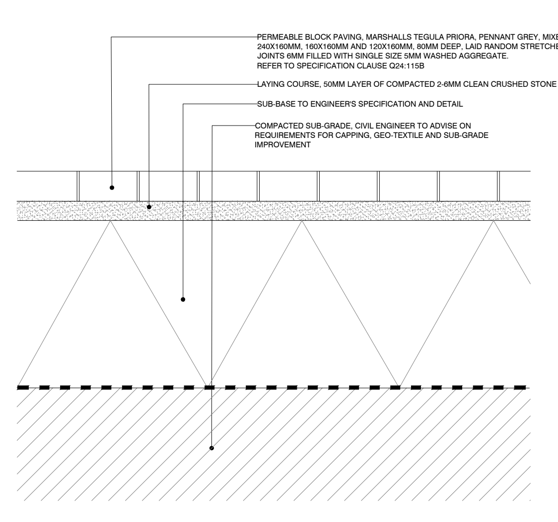
003 PERMEABLE BLOCK PAVING TO FOOTPATHS TYPE 1 SECTION SCALE - 1:10
