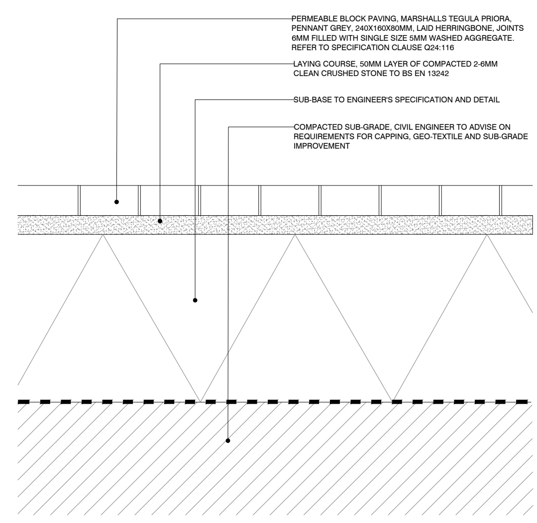
001 PERMEABLE BLOCK PAVING TO PARKING SPACES SECTION SCALE - 1:10
