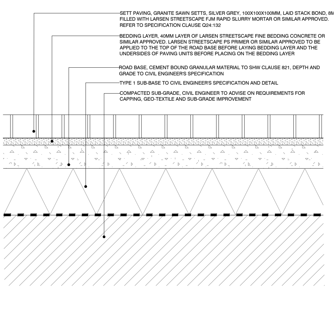
005 SETT PAVING TO ROAD ENTRANCE POINTS SECTION SCALE - 1:10
