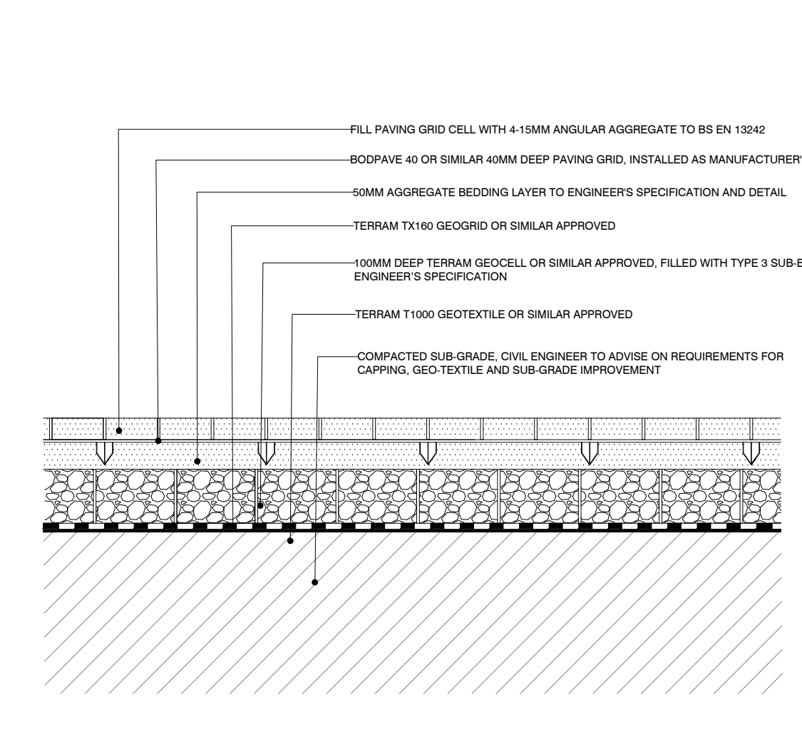
010 PARKING SPACE SURFACE WITHIN ROOT PROTECTION ZONES SECTION SCALE - 1:10
