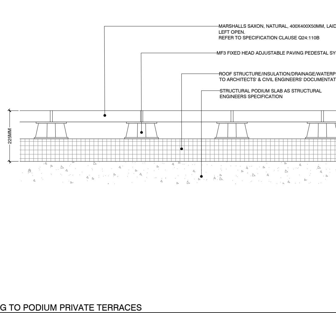
015 FLAG PAVING TO PODIUM PRIVATE TERRACES SECTION SCALE - 1:10
