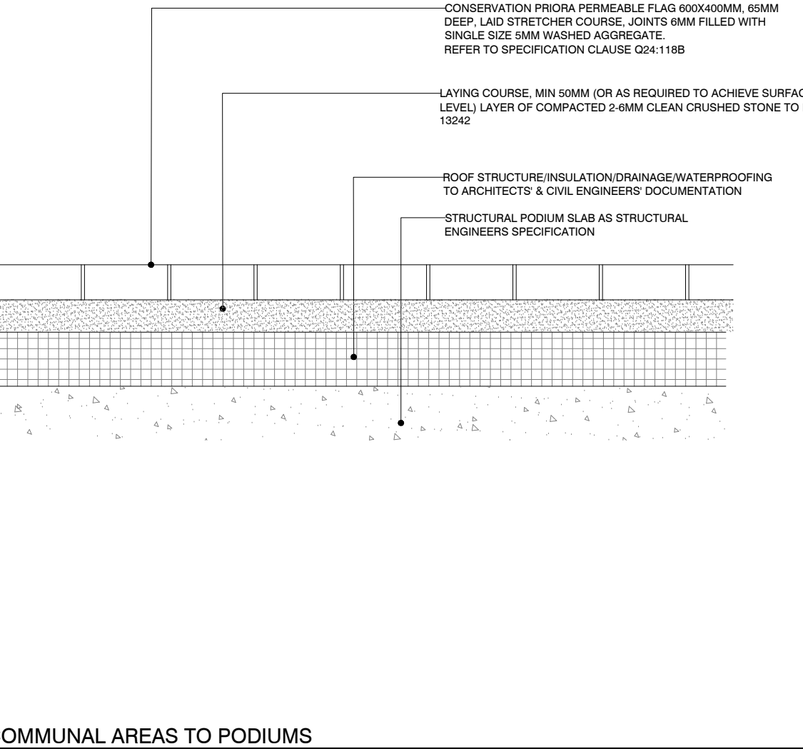
014 PAVING TO COMMUNAL AREAS TO PODIUMS SECTION SCALE - 1:10
