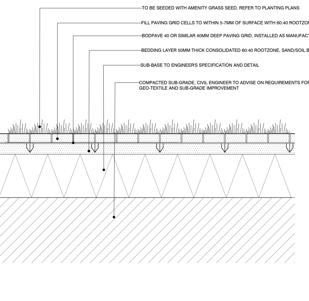
009 GRASS REINFORCEMENT SYSTEM SECTION SCALE - 1:10
