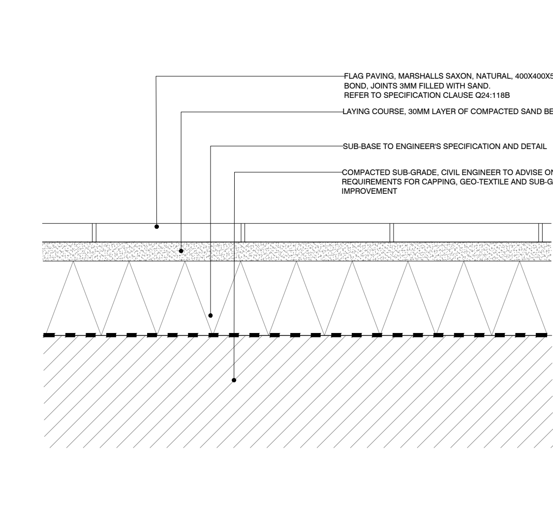
007 FLAG PAVING TO PRIVATE TERRACES SECTION SCALE - 1:10
