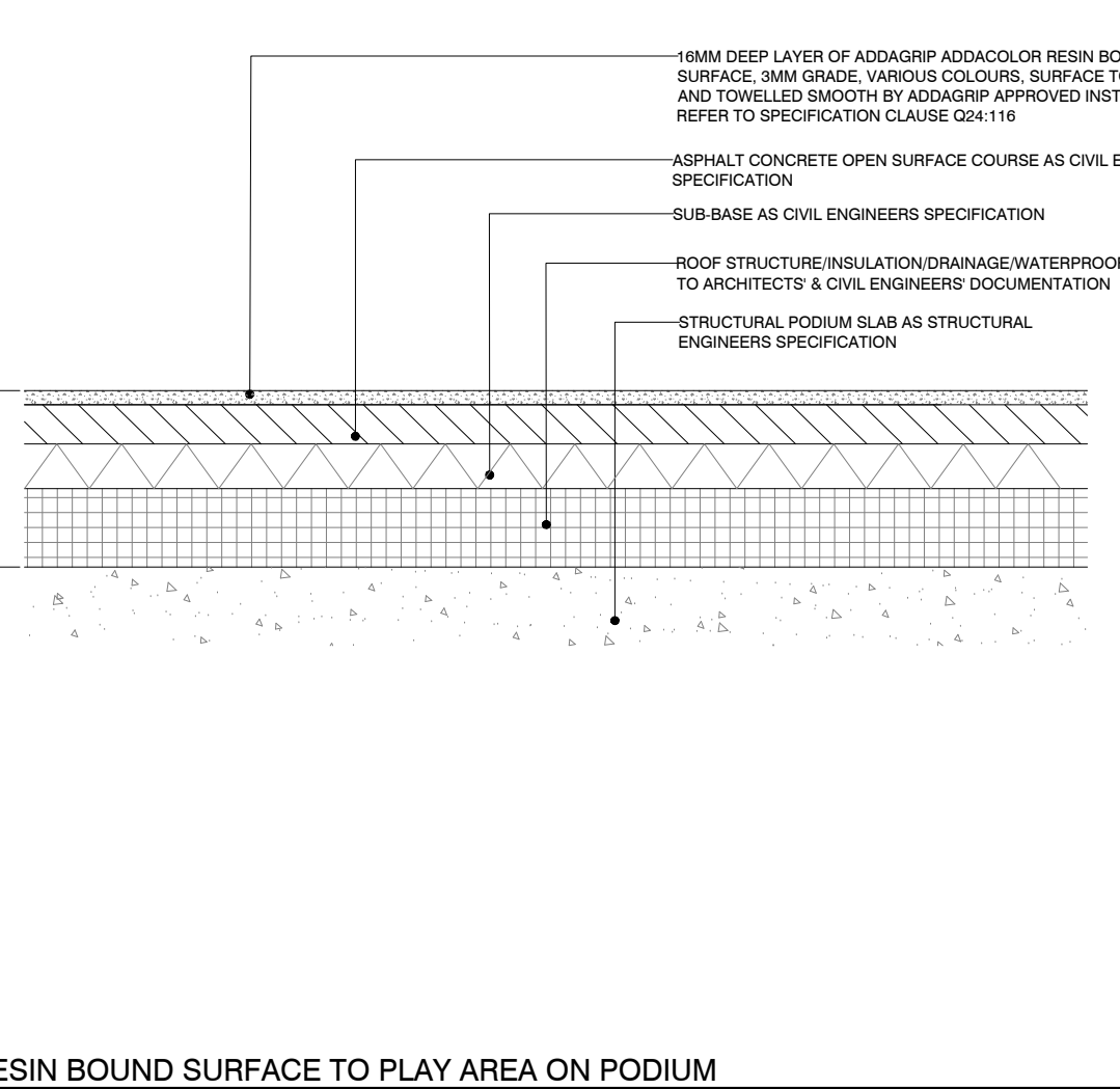
013 COLOURED RESIN BOUND SURFACE TO PLAY AREA ON PODIUM SECTION SCALE - 1:10
