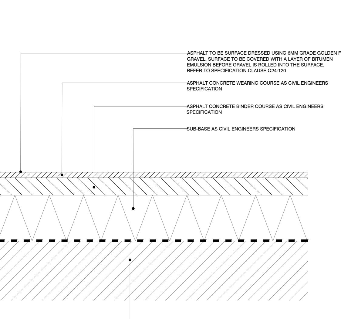
011 TOP DRESSED ASPHALT SURFACE SECTION SCALE - 1:10
