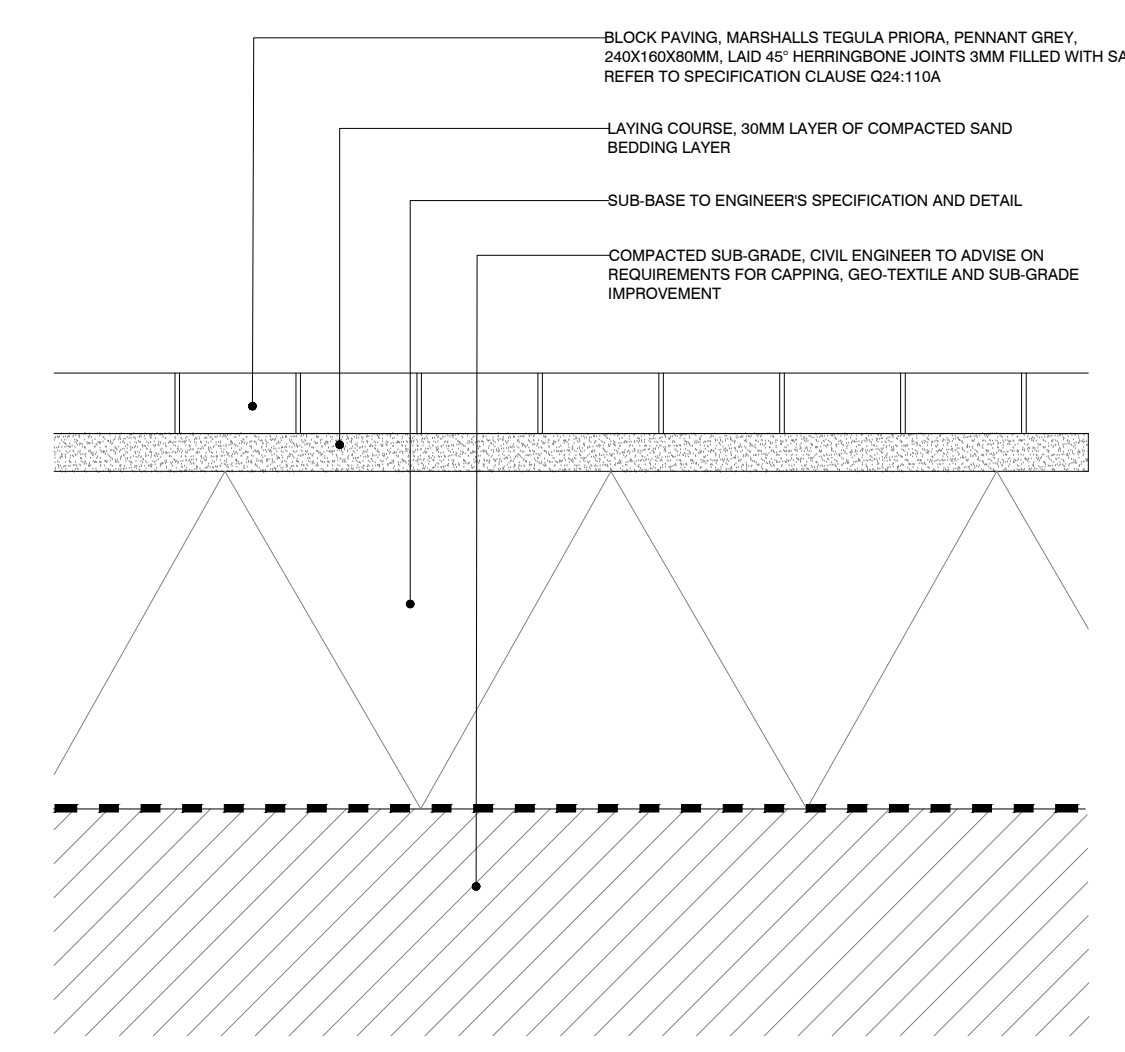
002 BLOCK PAVING TO ROADS SECTION SCALE - 1:10
