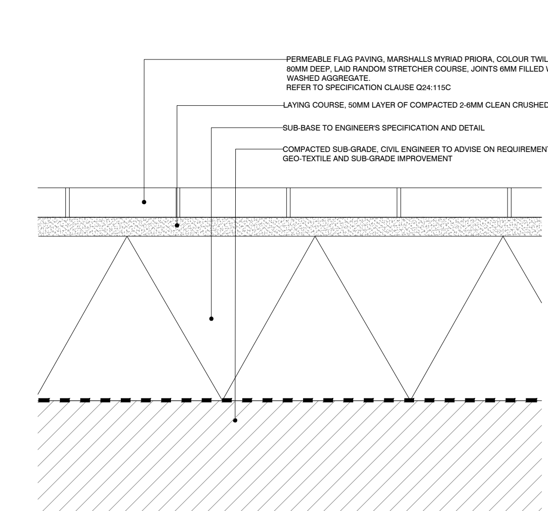
006 PERMEABLE FLAG PAVING TO BUILDING ENTRANCE AREAS SECTION SCALE - 1:10
