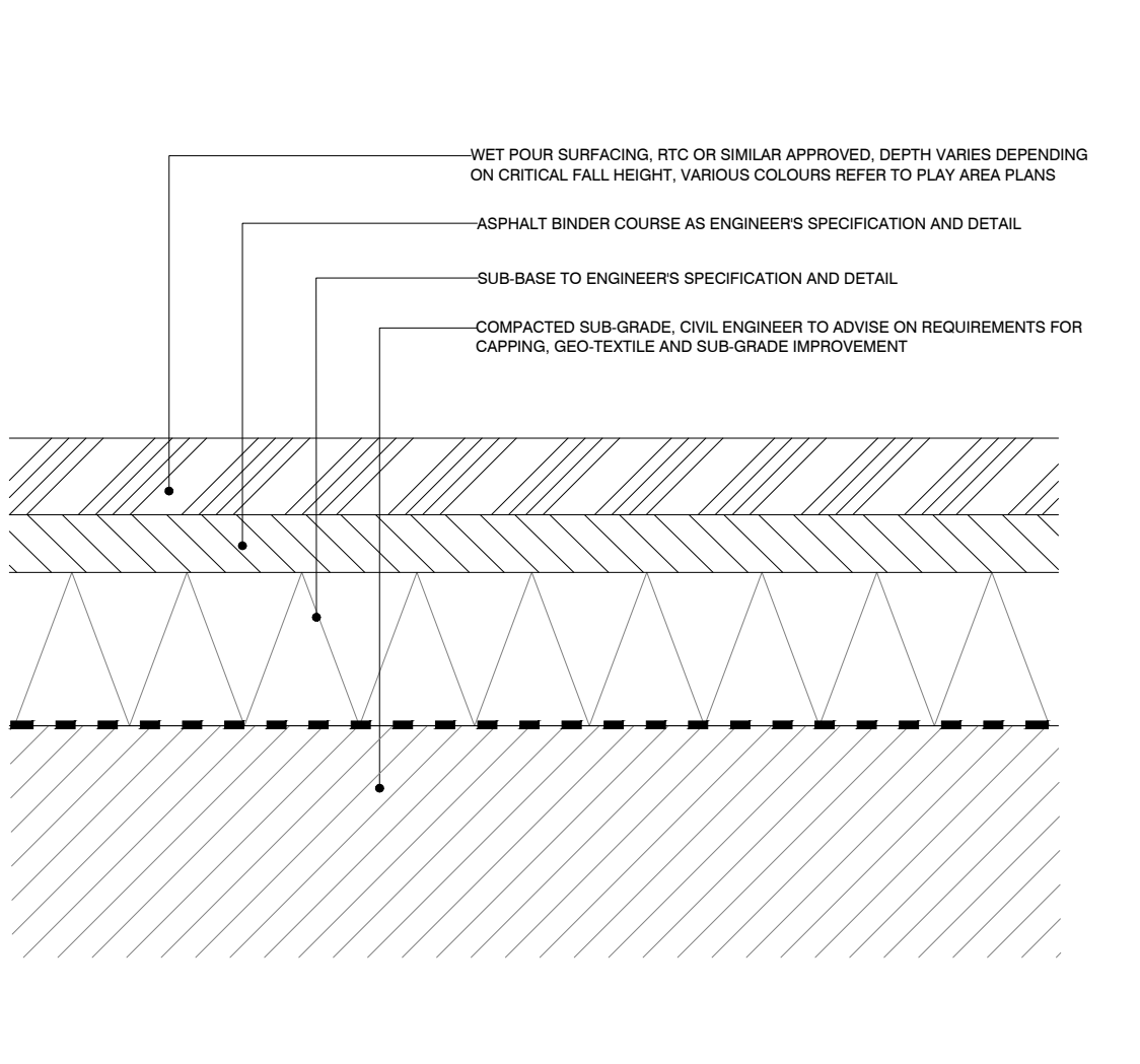
008 PLAY AREA SURFACE SECTION SCALE - 1:10
