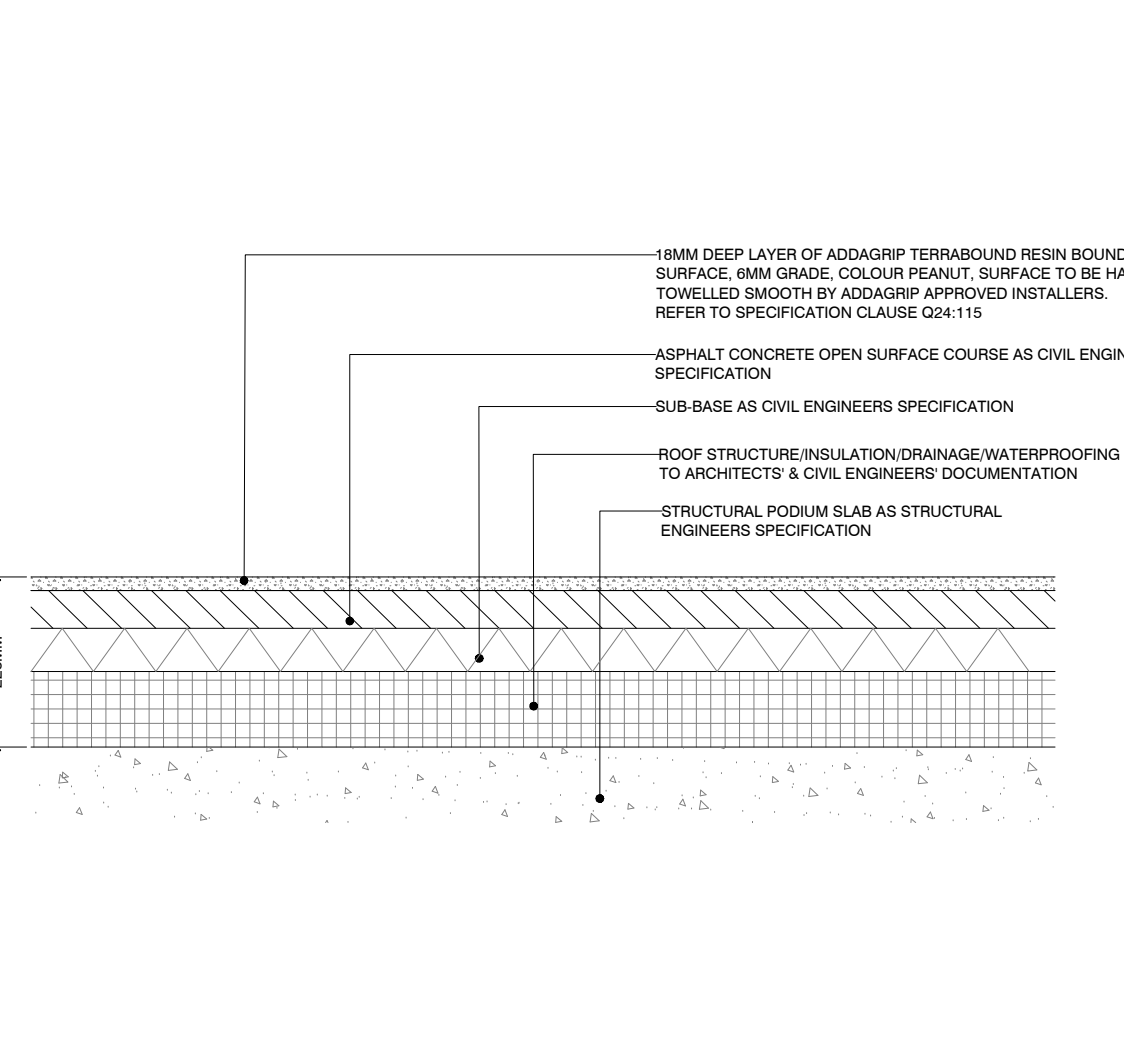
012 RESIN BOUND GRAVEL TO PODIUM SECTION SCALE - 1:10
