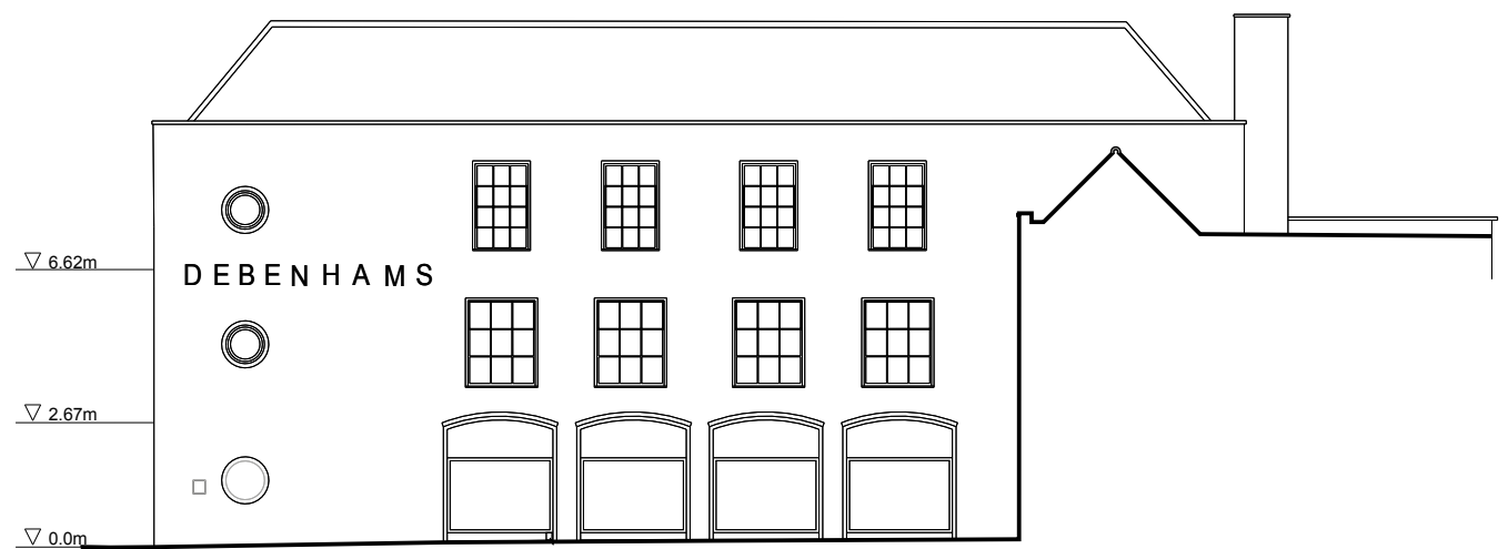
ELEVATION 3 (WEST ELEVATION)
