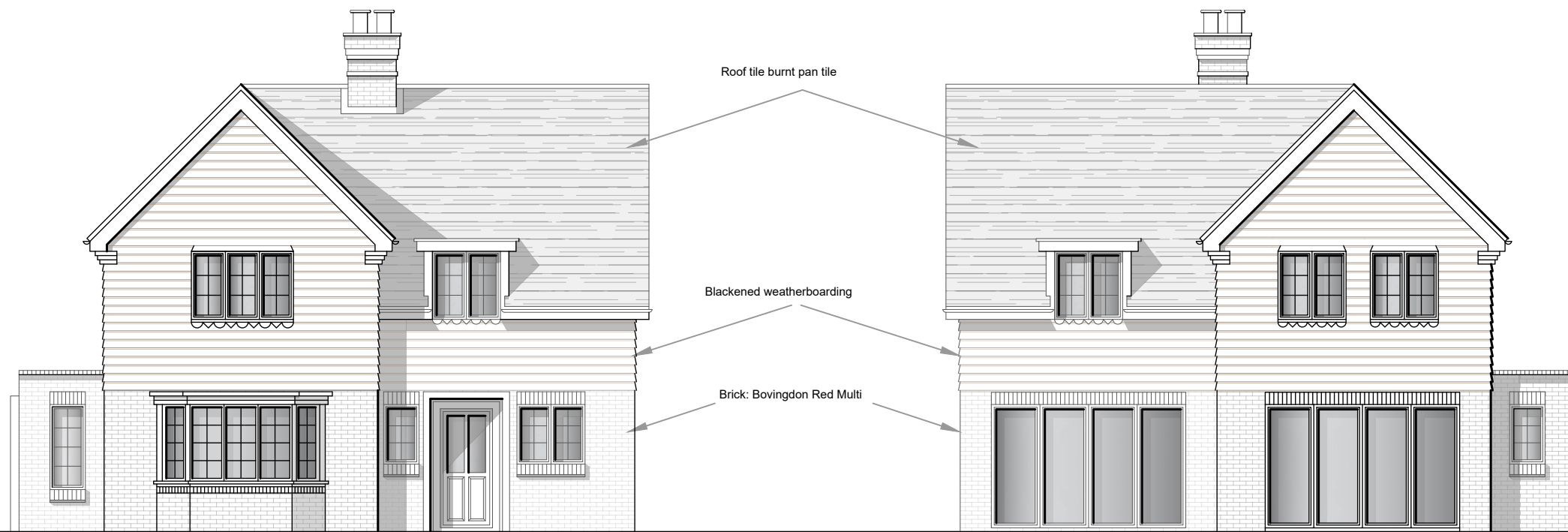
Front Elevation
