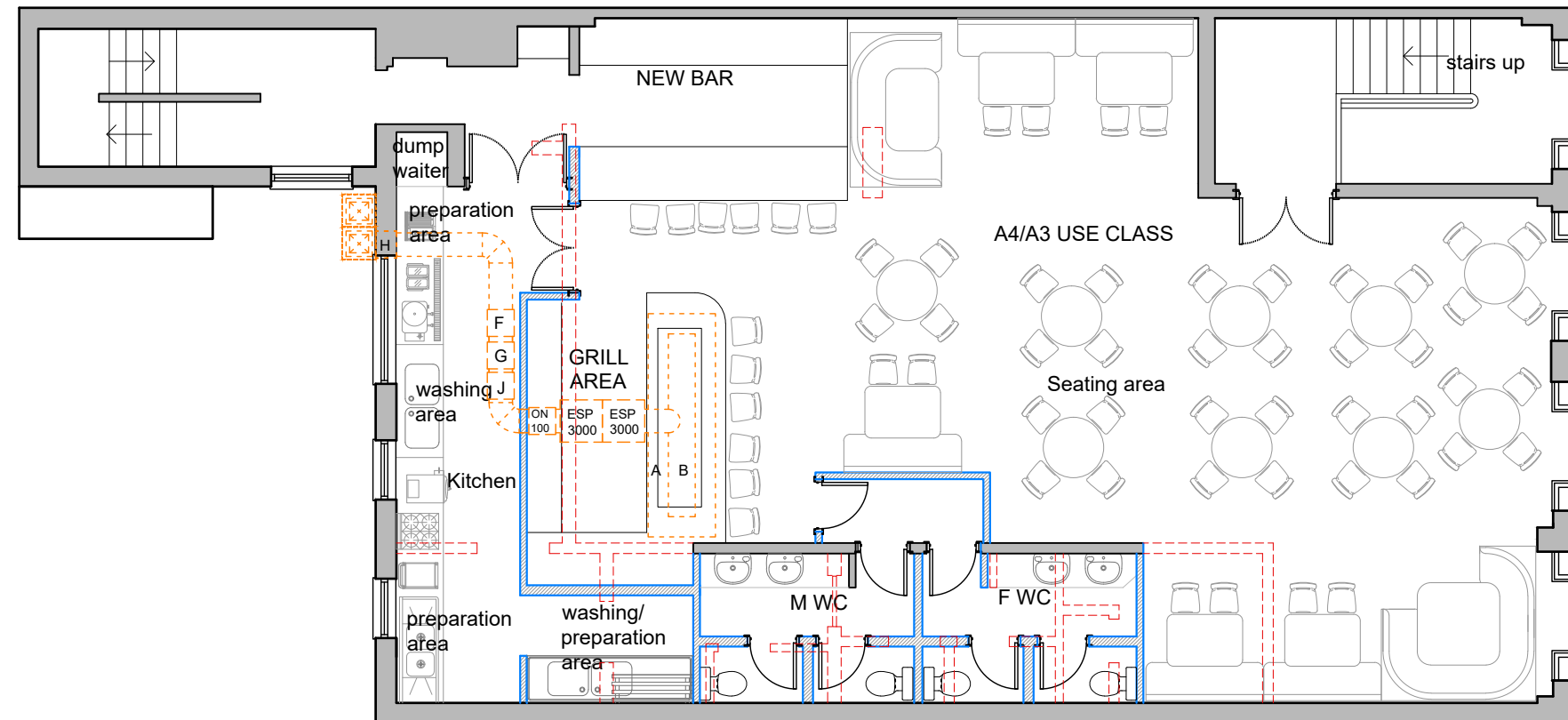
PROPOSED 1ST FLOOR PLAN
