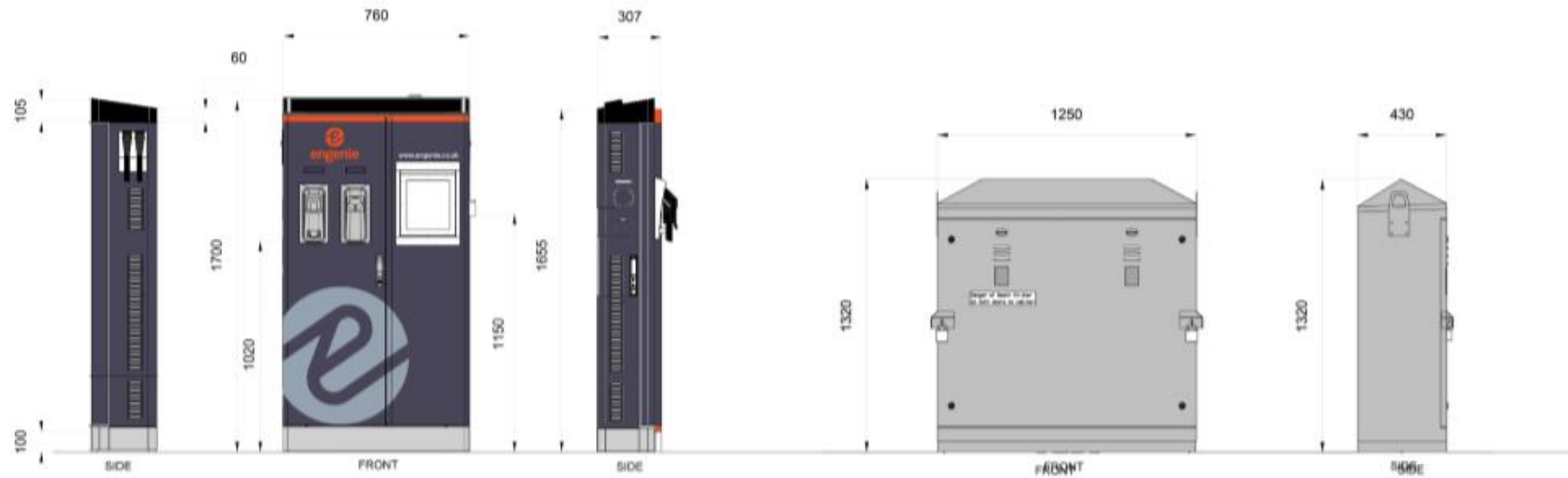
AAB CHARGER EV EQUIPMENT DETAIL ELEVATIONS
