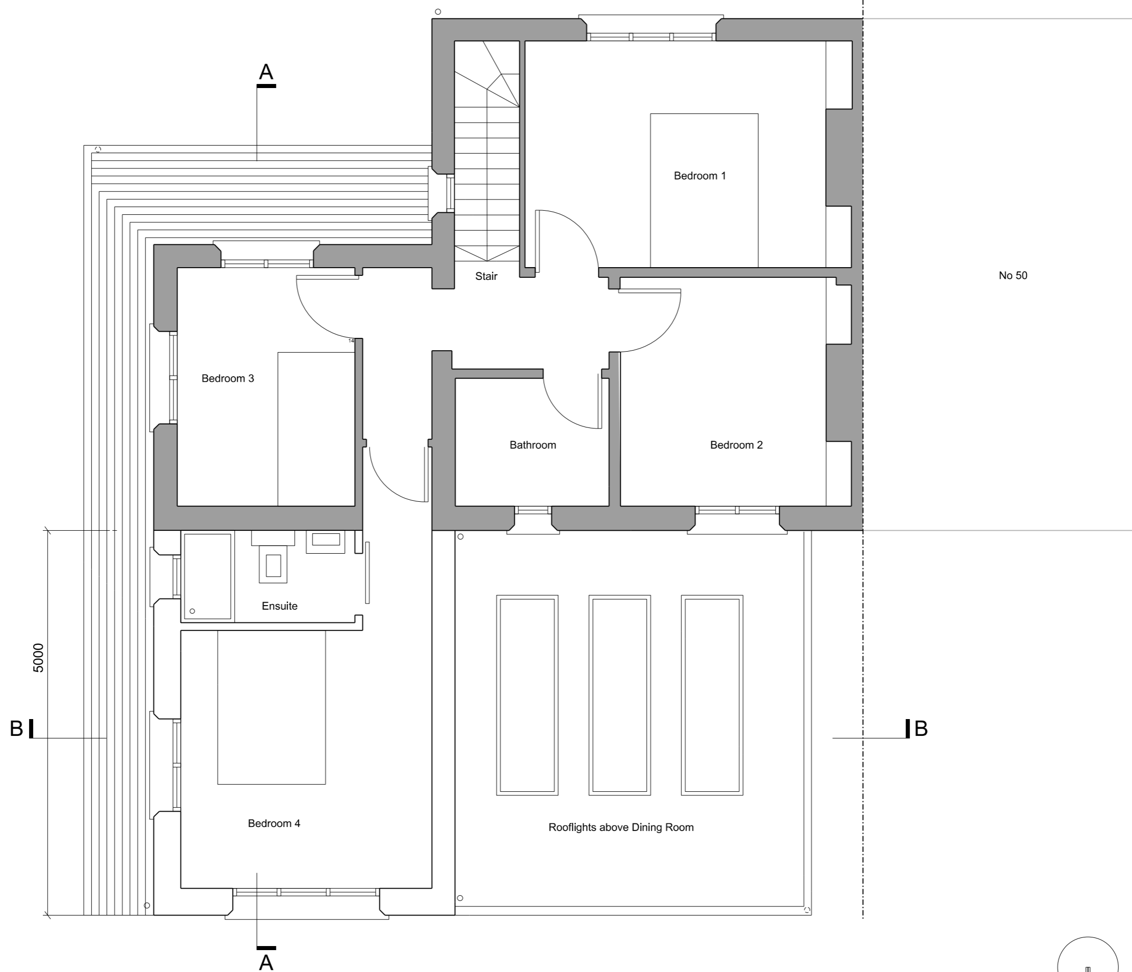
PROPOSED FIRST FLOOR PLAN - 1:50 @ A3
