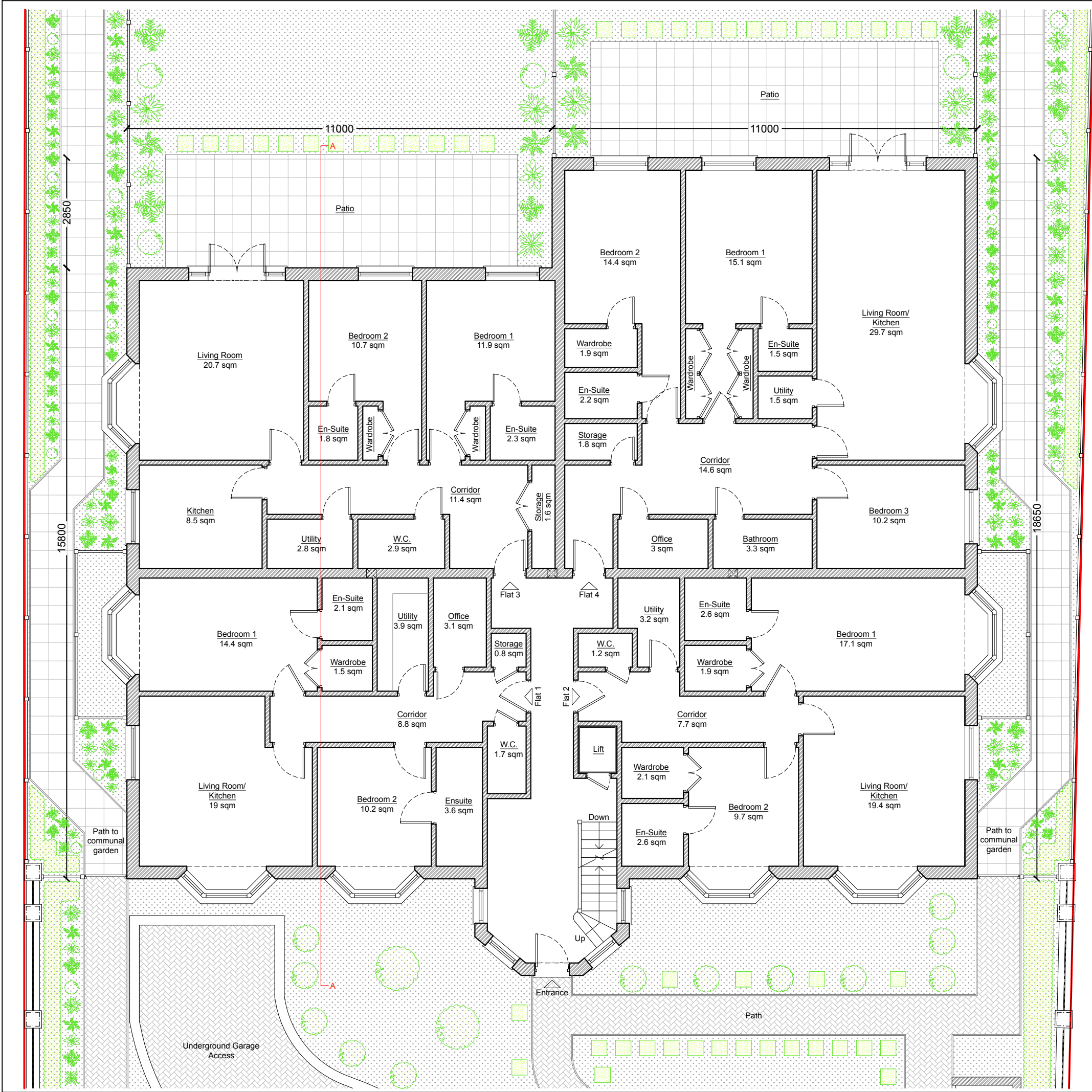
Ground Floor Plan As Proposed - Scale 1:100
