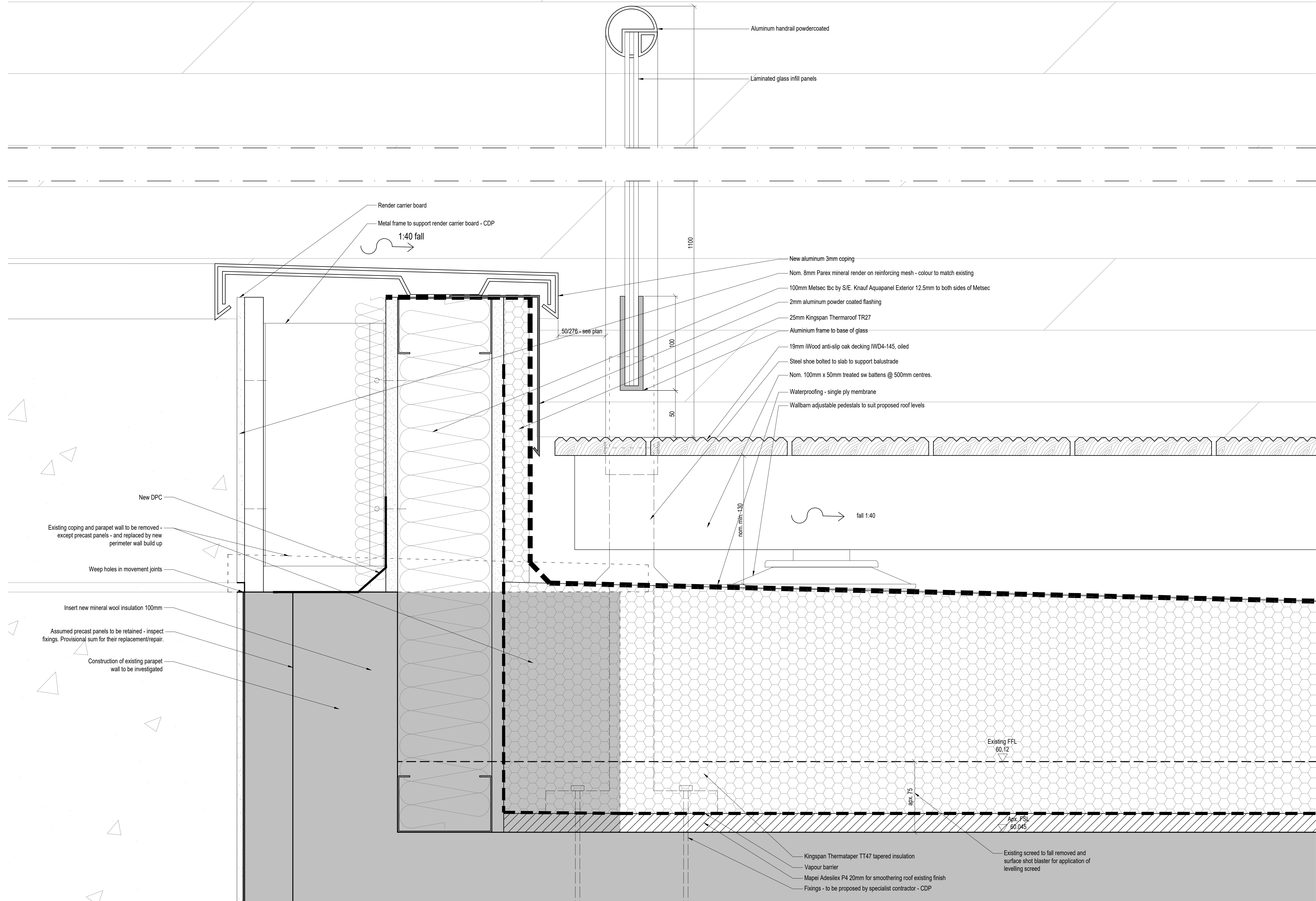
Third Floor Baluster detail SCALE: 1:2@A1
