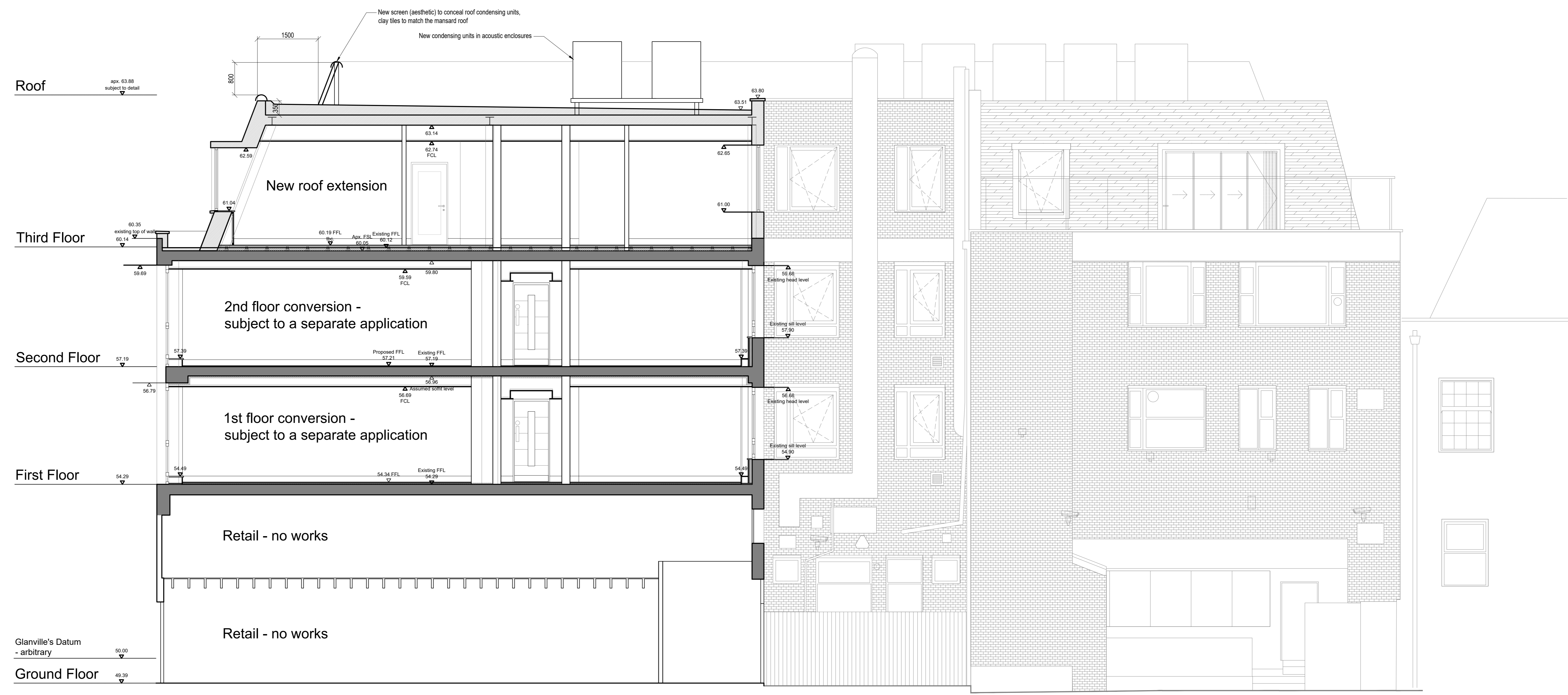
SECTION THROUGH BUILDING TO SHOW CONDENSING UNITS IN ENCLOSURES AND SCREEN TO CONCEAL THEM SCALE: 1:50 @ A0
