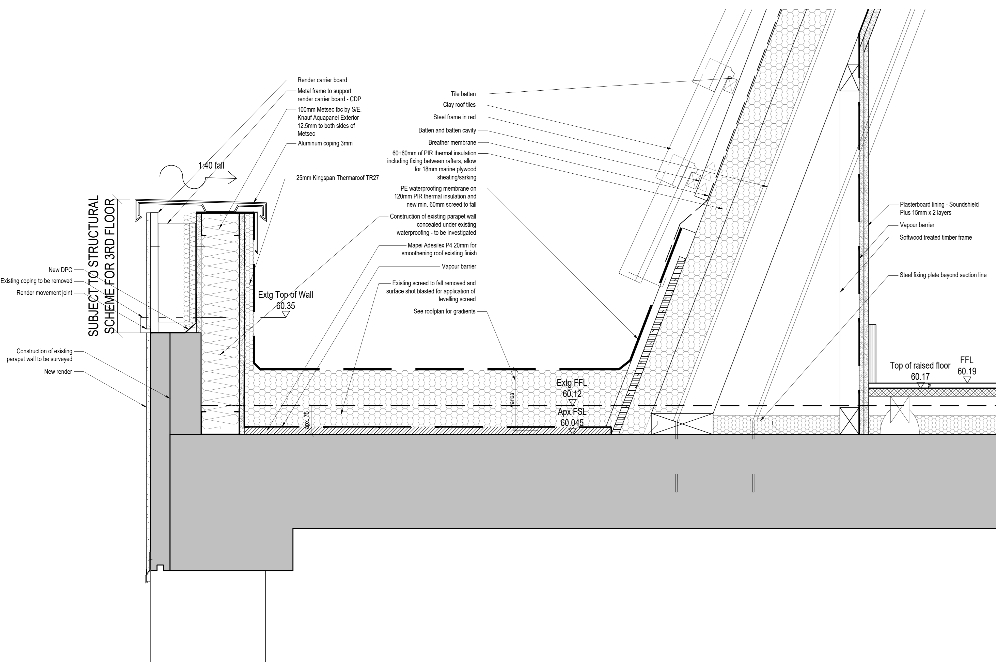
TYPICAL ROOF DETAILS SCALE: 1:5 @ A0
