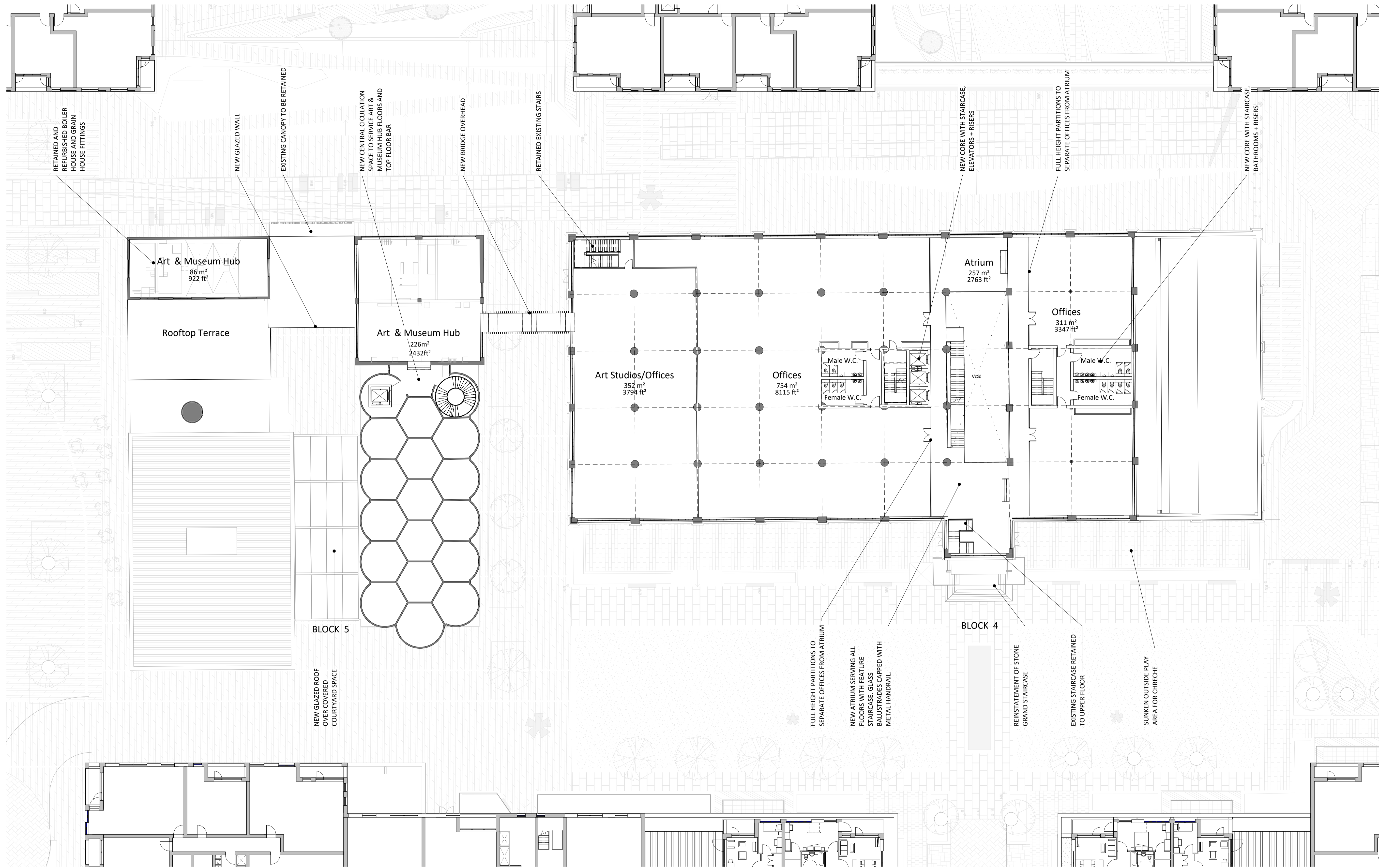
1 GIA - Second Floor 1:200 @A1
