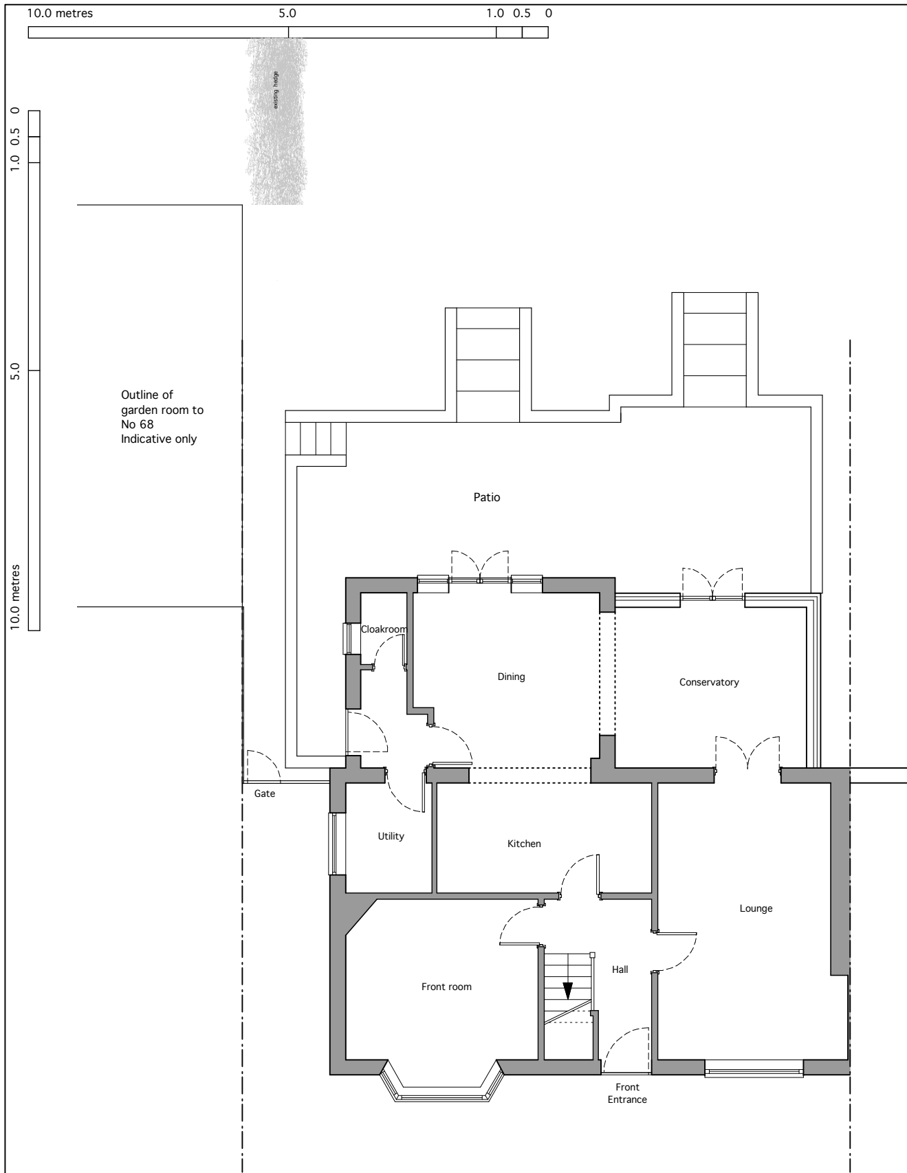
1 66 Brockwood Lane Existing Ground Floor Plan 1:100
