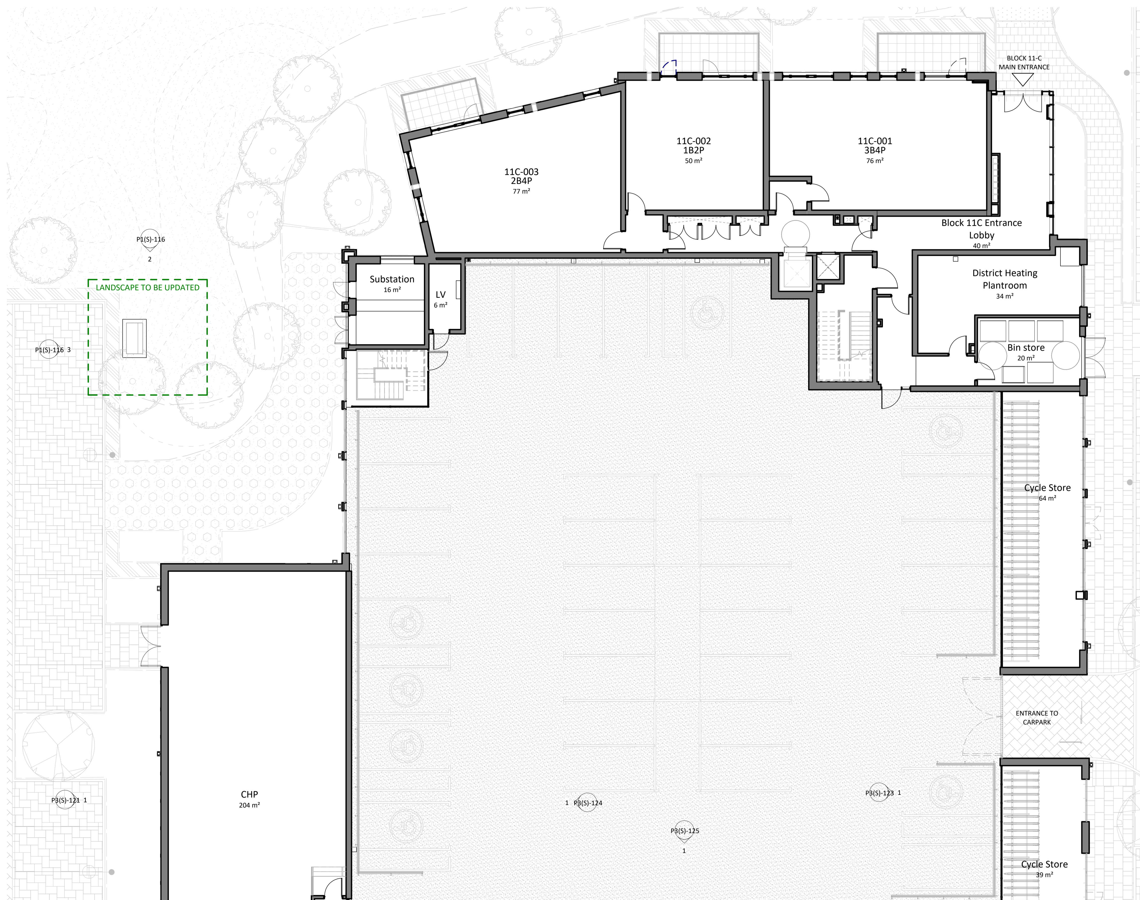
1 Block 11 - Ground Floor - Block C 1 : 100 @A1
