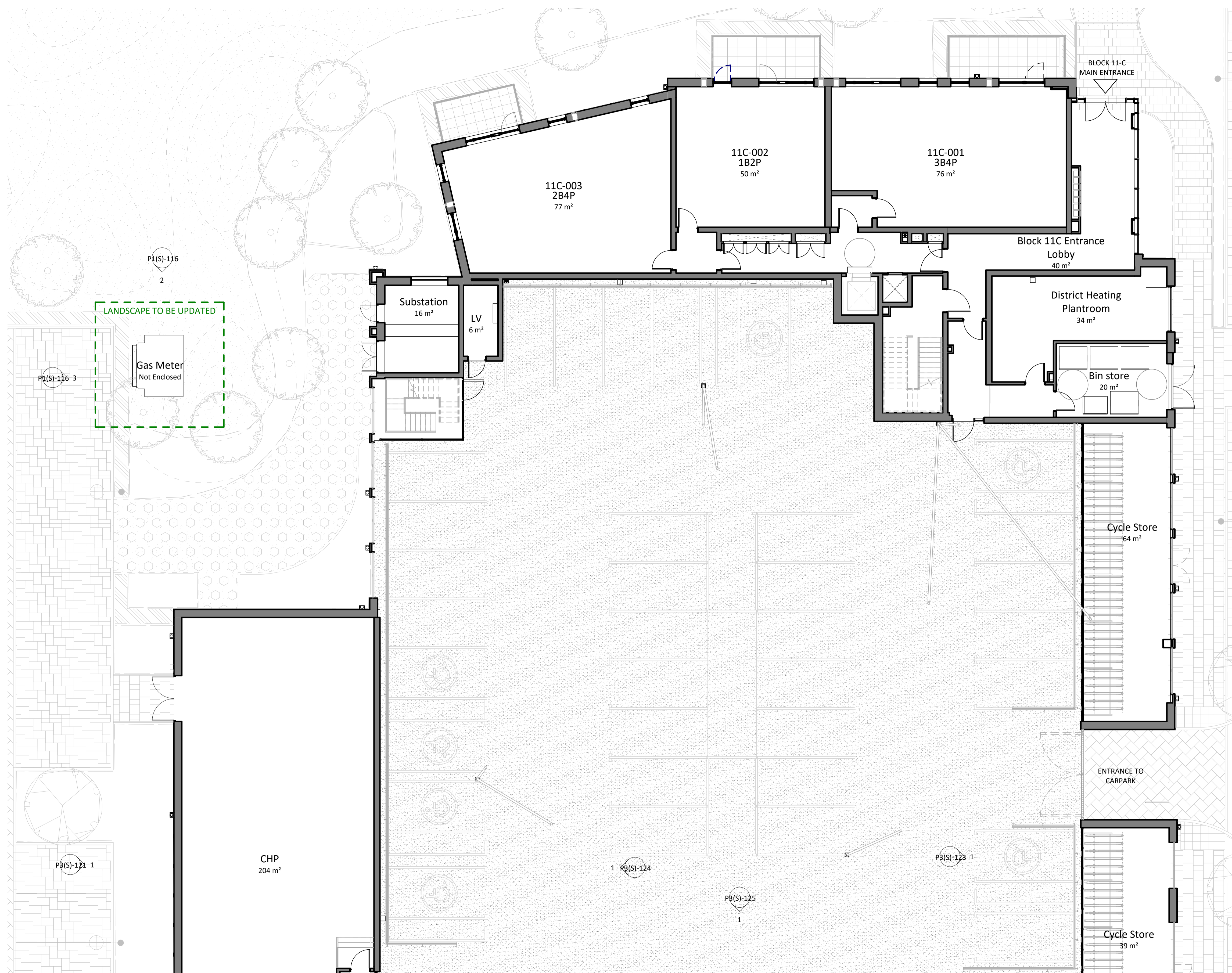
1 Block 11 - Ground Floor - Block C
