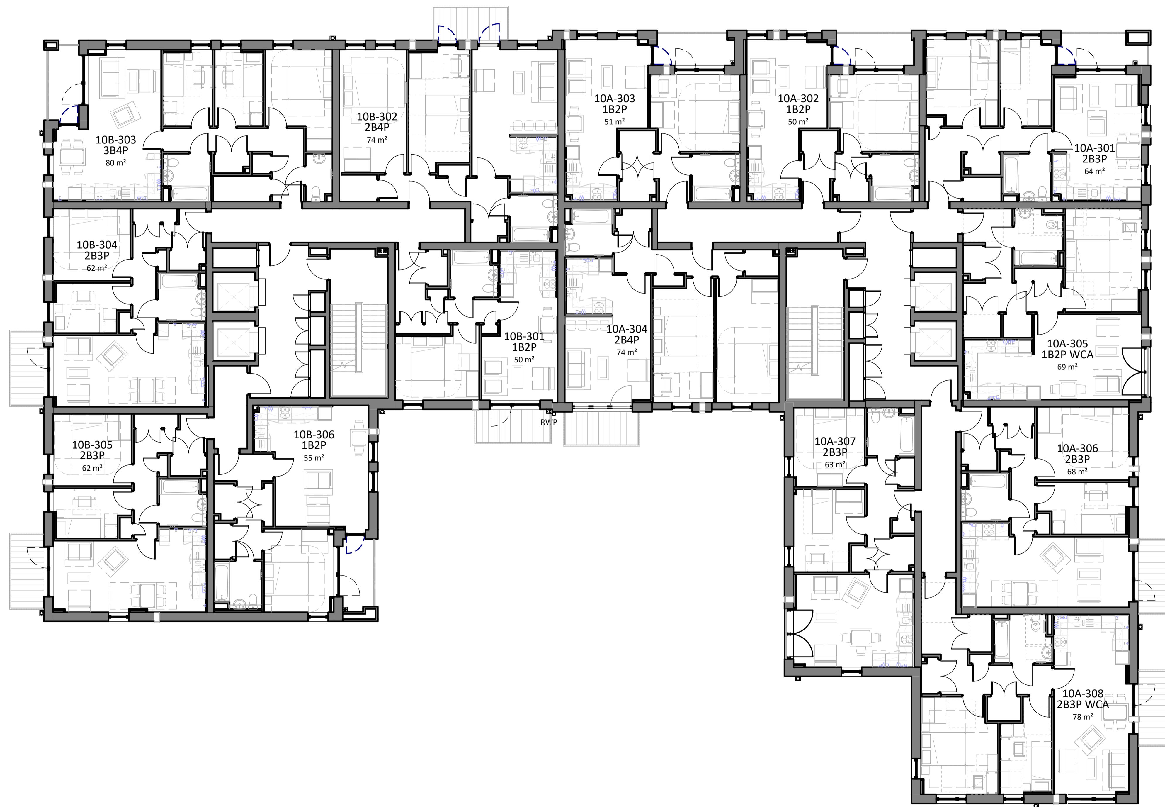
1 Block 10 A/B Typical Floor Plan 1 : 100 @A1
