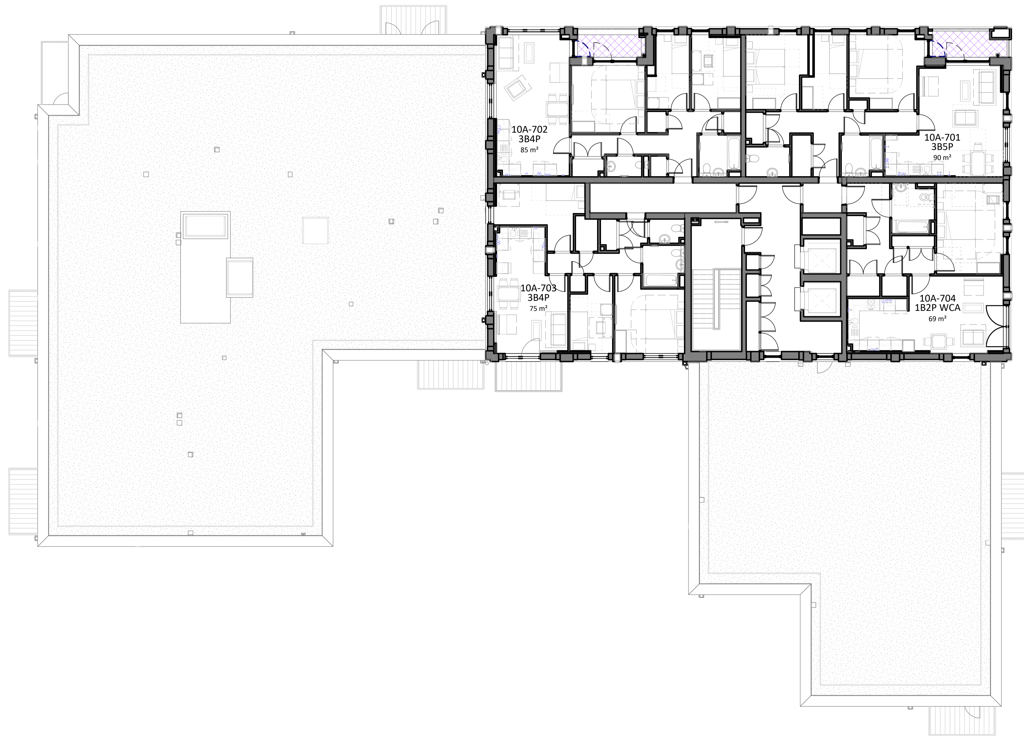
1 Block 10 A/B Top Floor Plan 1 : 100 @A1
