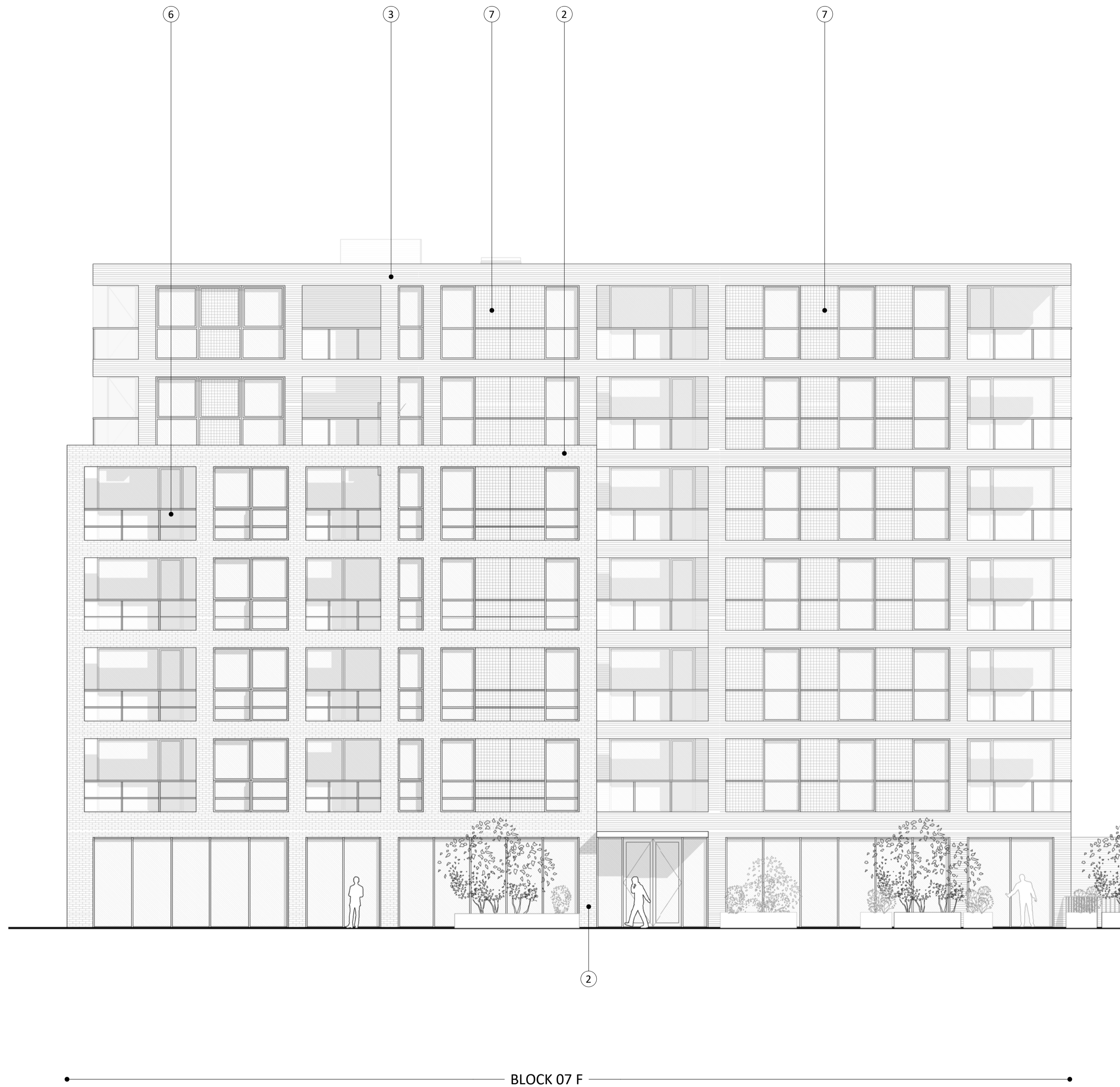
2 Block 07 (7F)-South Elevation 1 : 100 @A1
