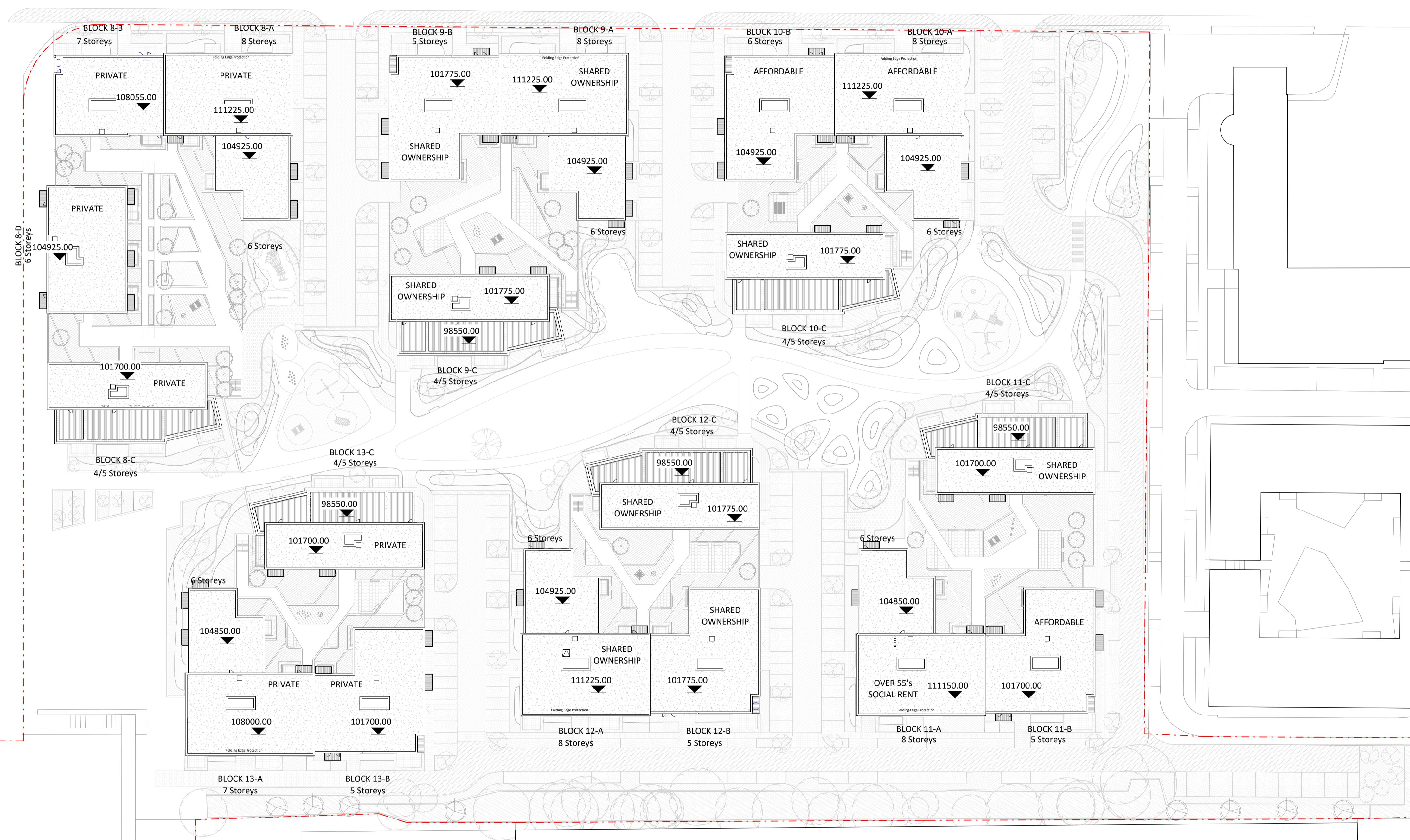
1 P0(S)-108 - Roof Level Plan 1 : 500 @A1
