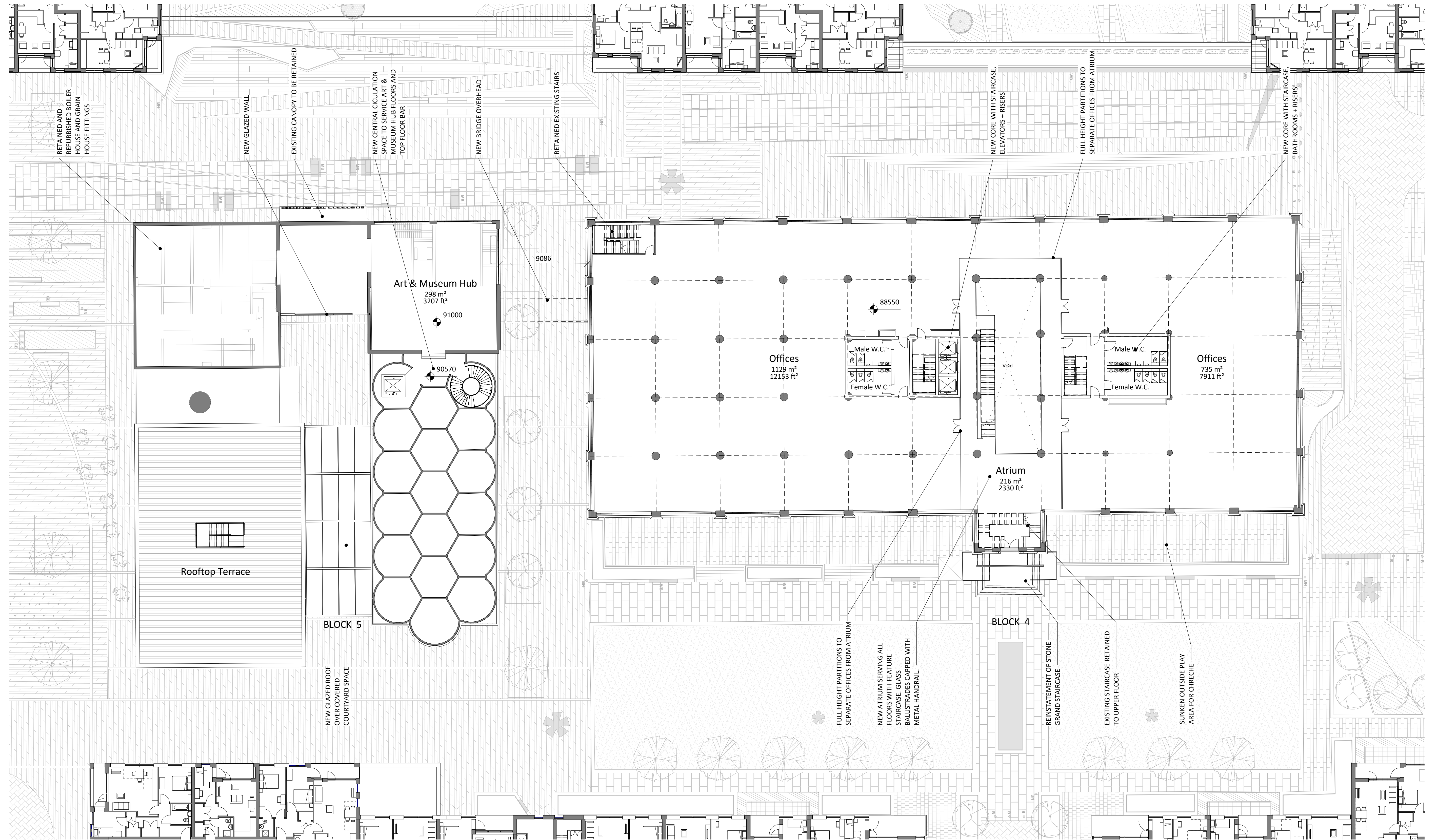
1 GIA - First Floor 1:200 @A1
