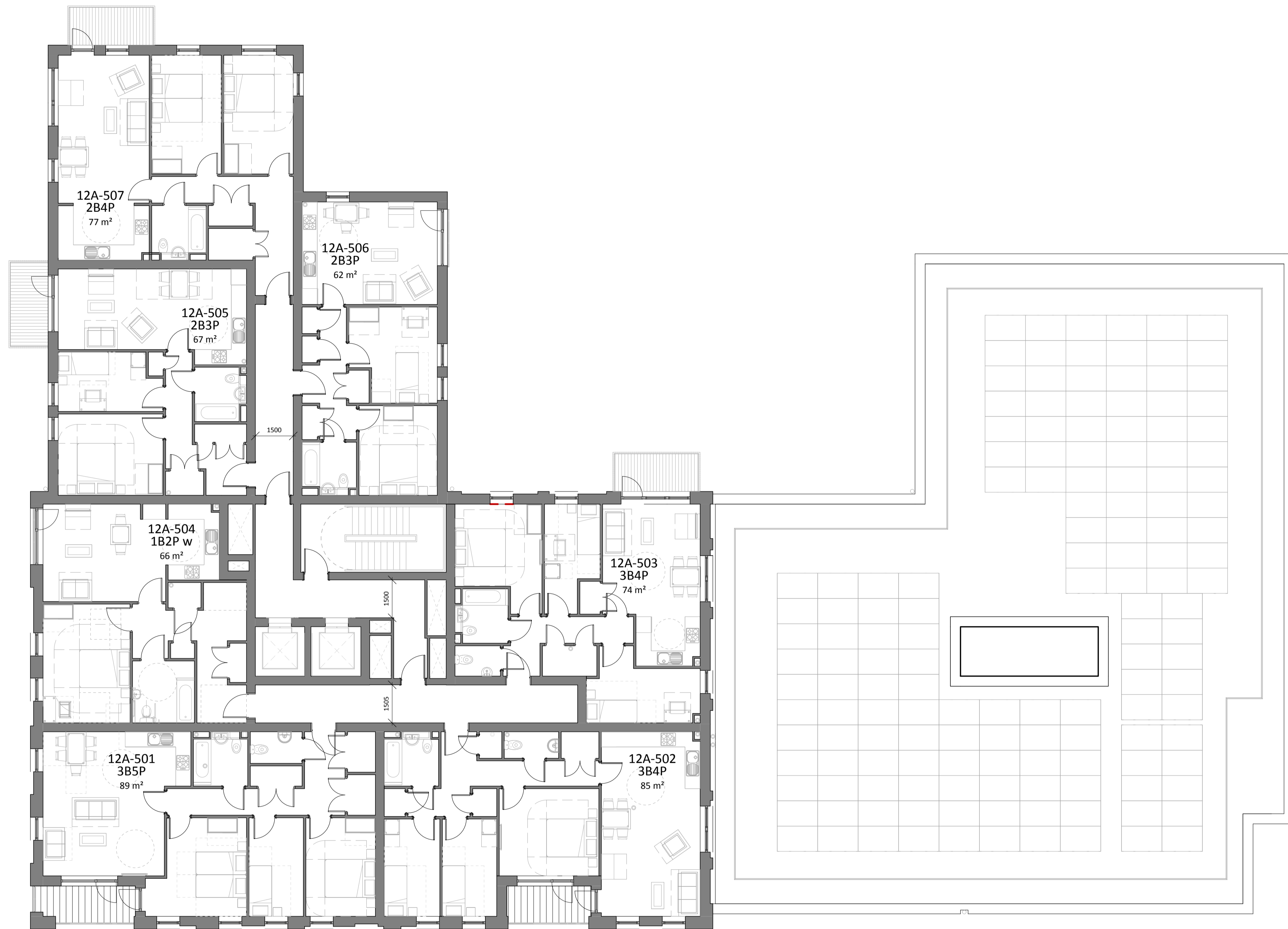
1 Block 12 - Fifth Floor Plan - Affordable 1:100 @A1
