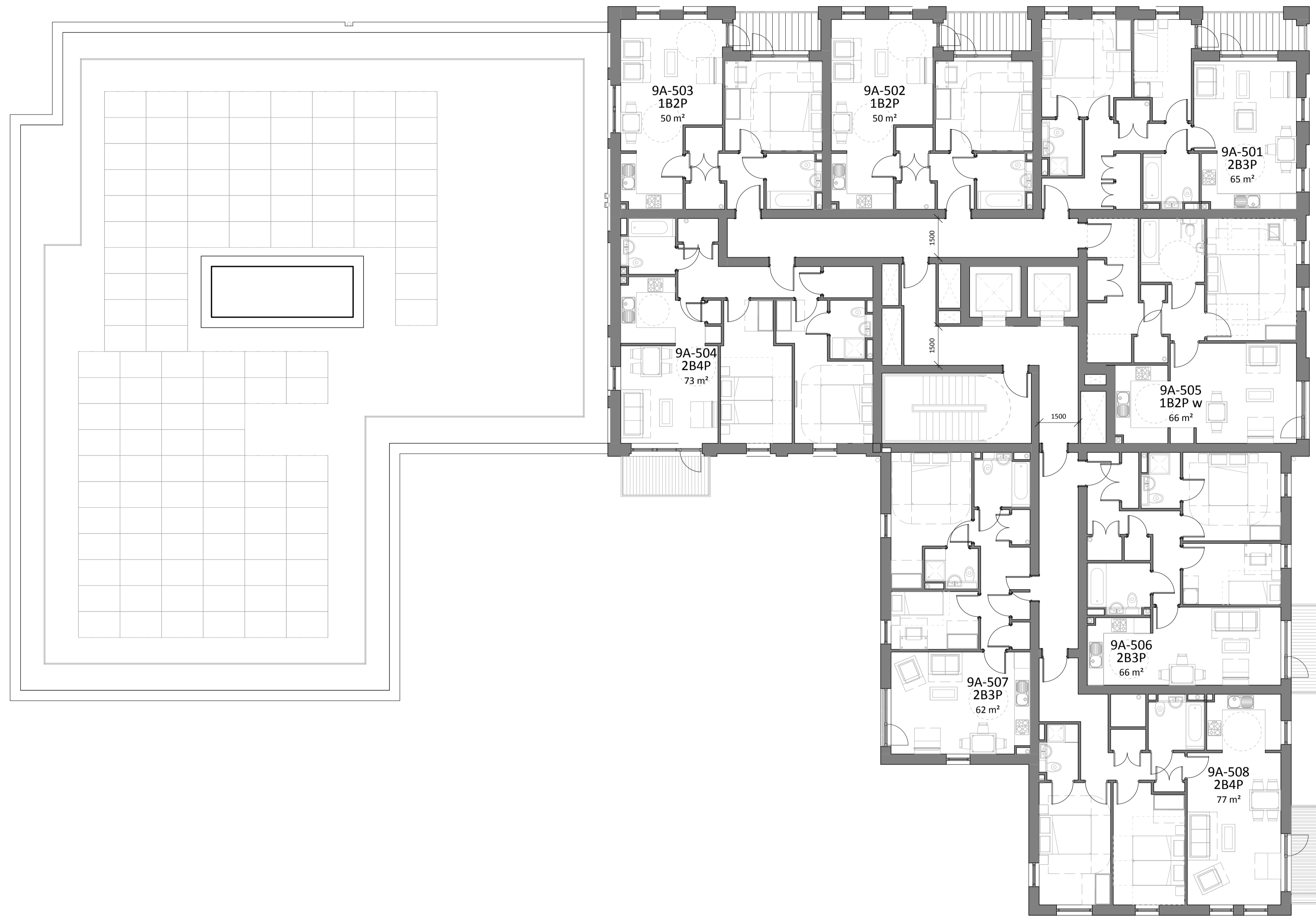
1 Block 5 - Fifth Floor Plan - Private 1 : 100 @A1
