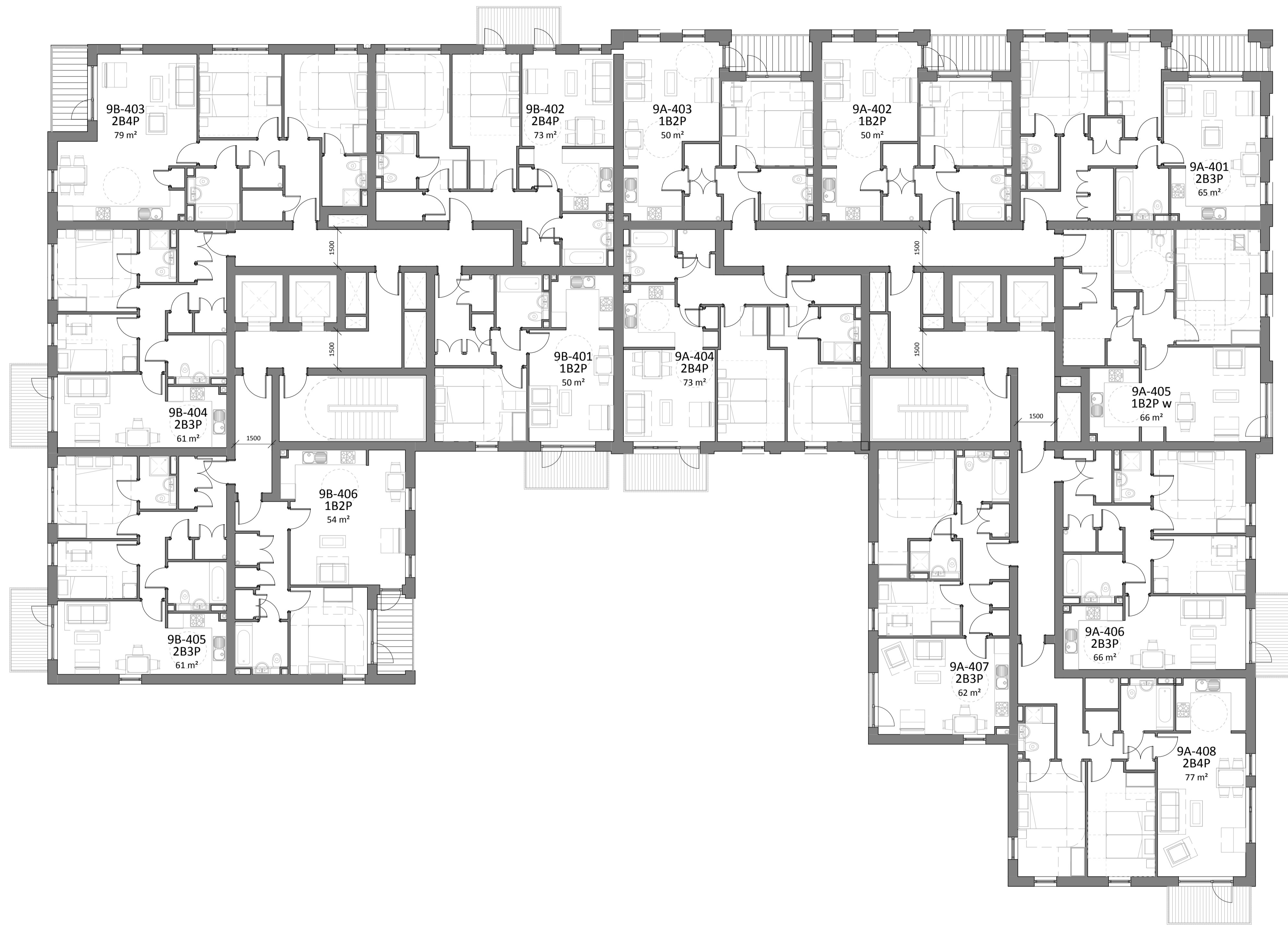
1 Block 9 - Fourth Floor Plan - Private 1 : 100 @A1
