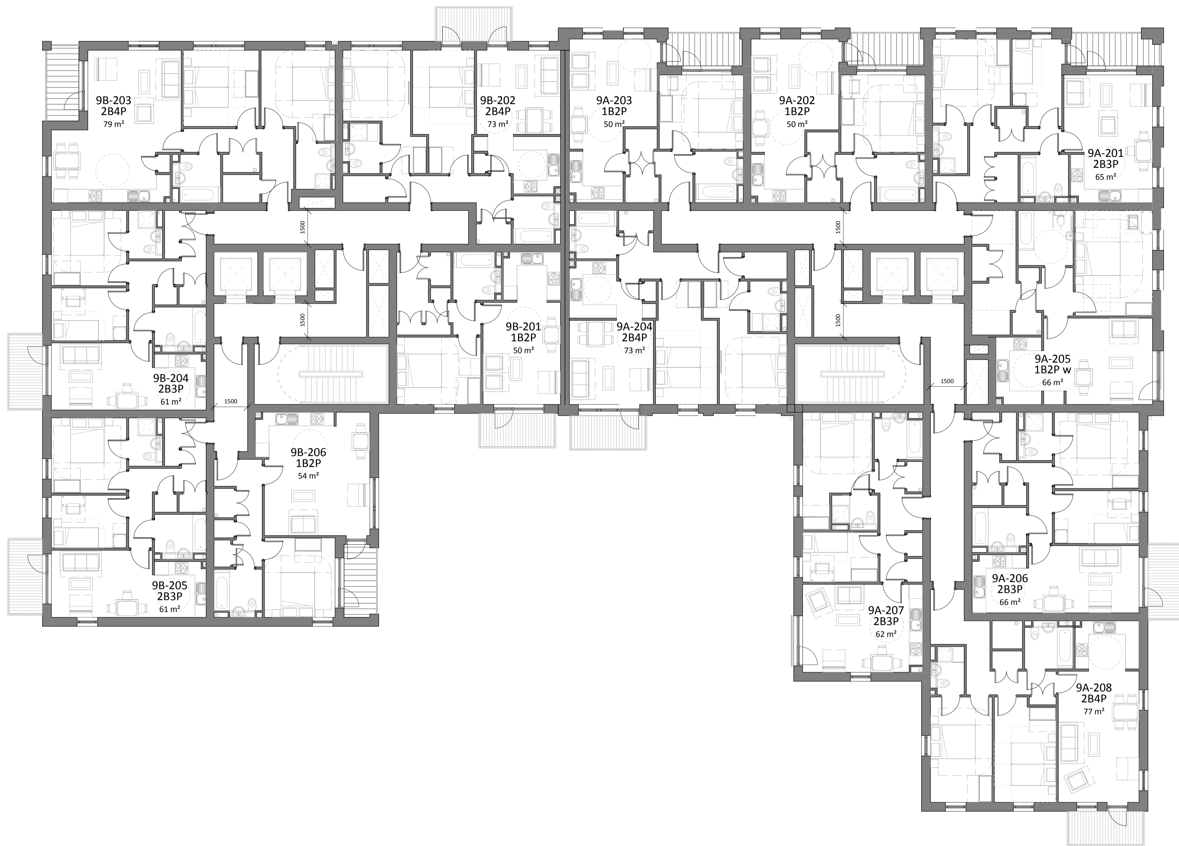
1 Block 9 - Typical Floor Plan - Private 1:100 @A1
