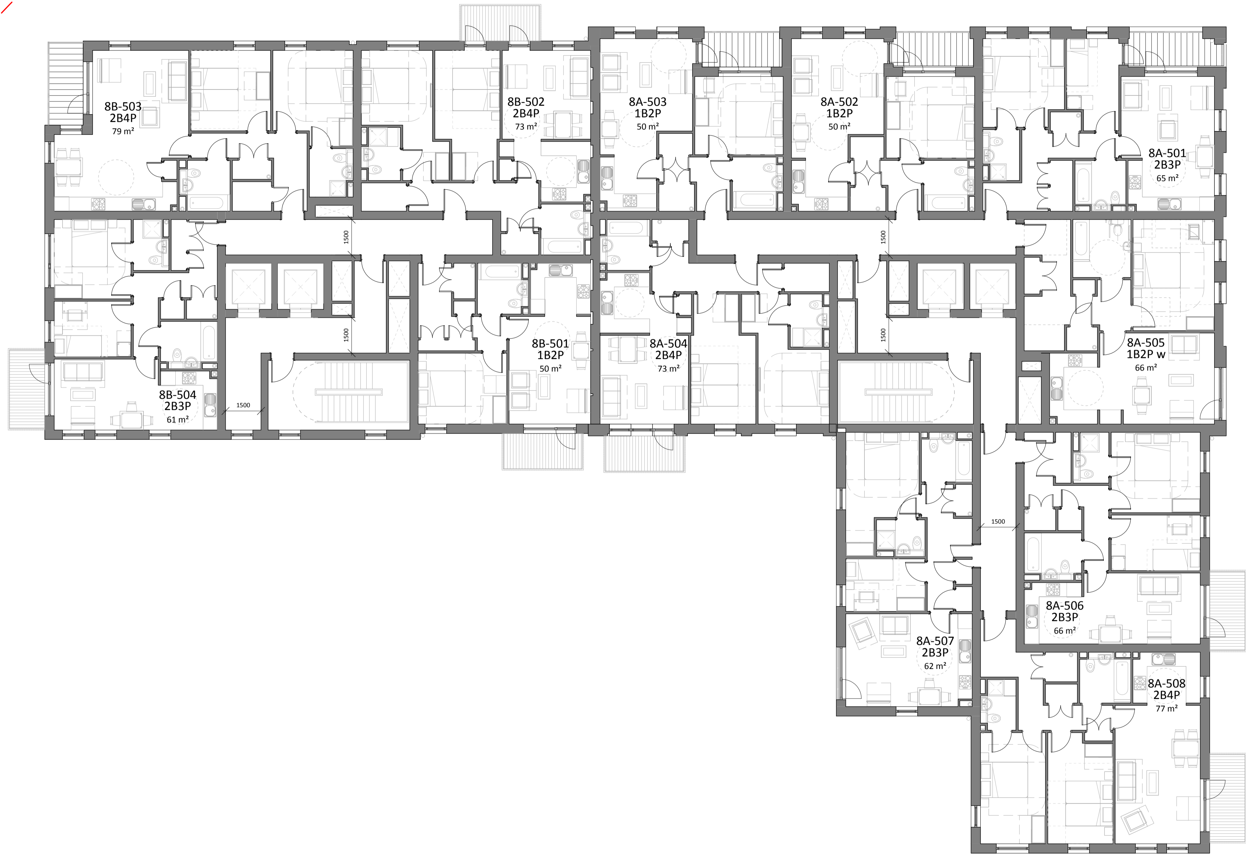
1 Block 8 A/B Fifth Floor - Private 1:100 @A1
