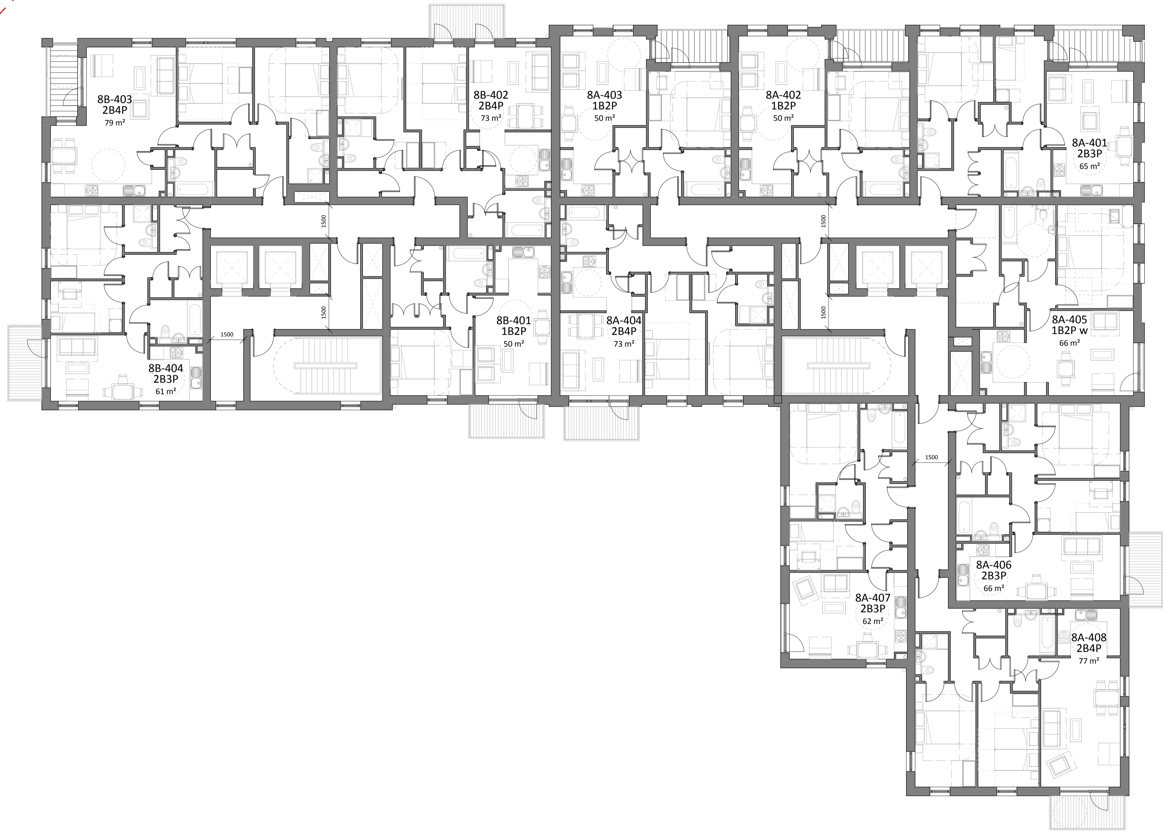
1 Block 8 A/B Fourth Floor - Private 1 : 100 @A1
