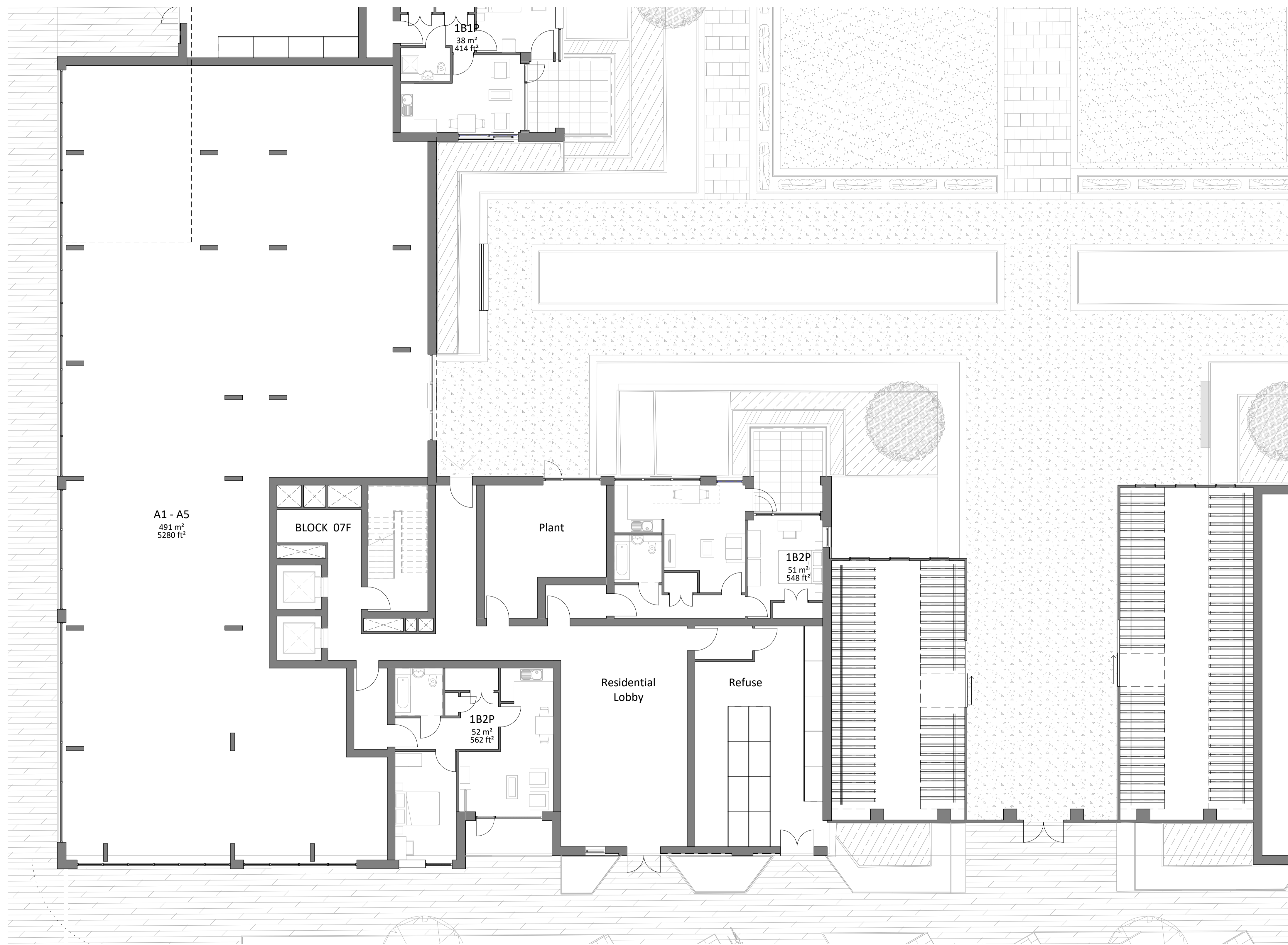
1 Block 07F - Ground Floor Plan 1 : 100 @A1
