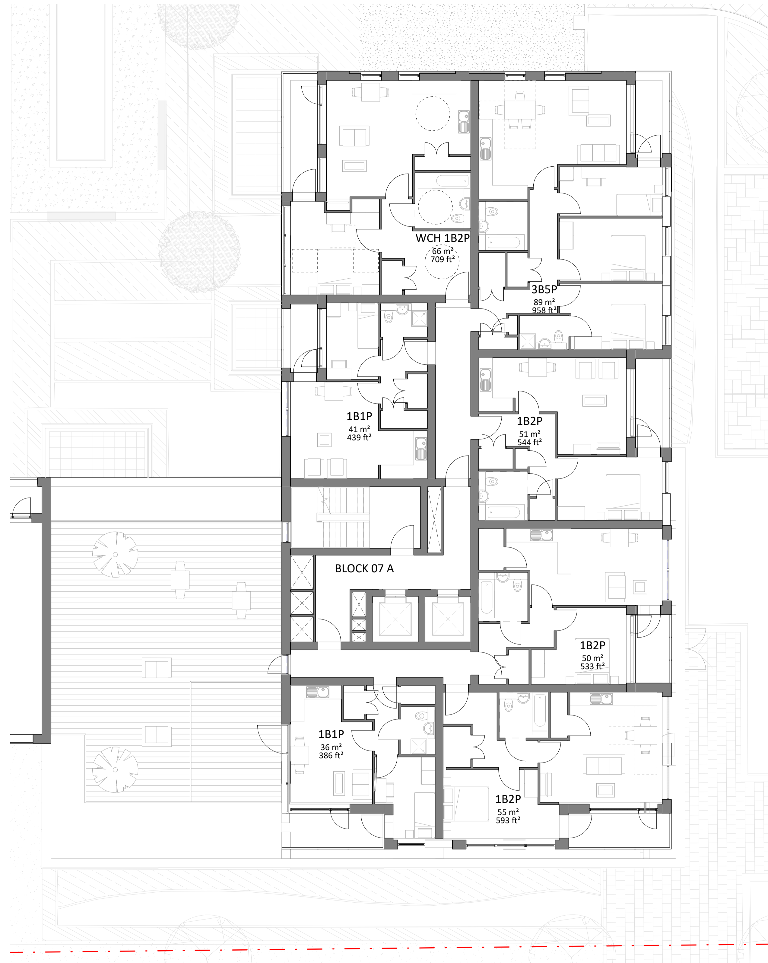
1 Block 07A Typical Top Floor Plan
