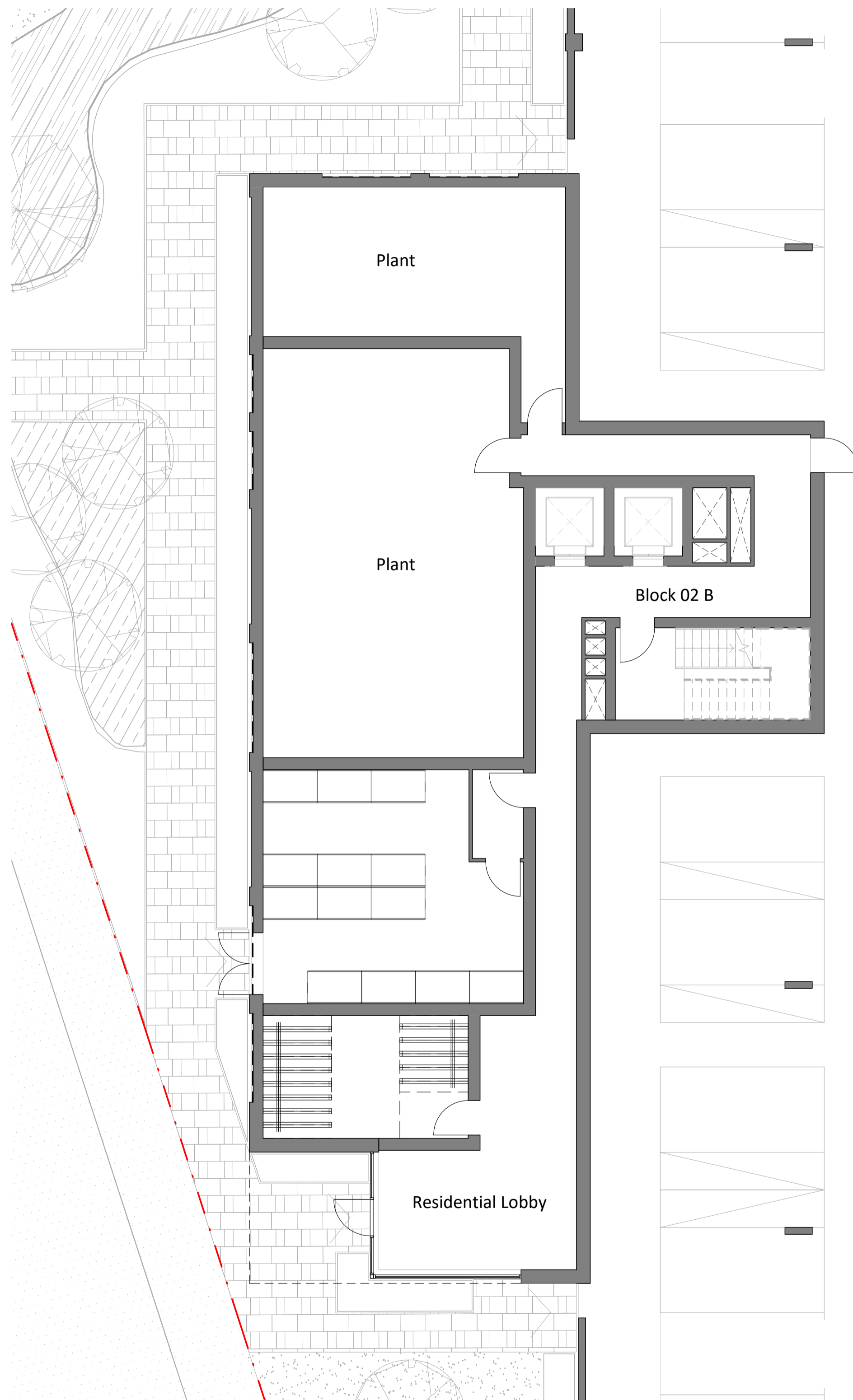
1 Block 02B - Ground Floor Plan 1 : 100 @A1
