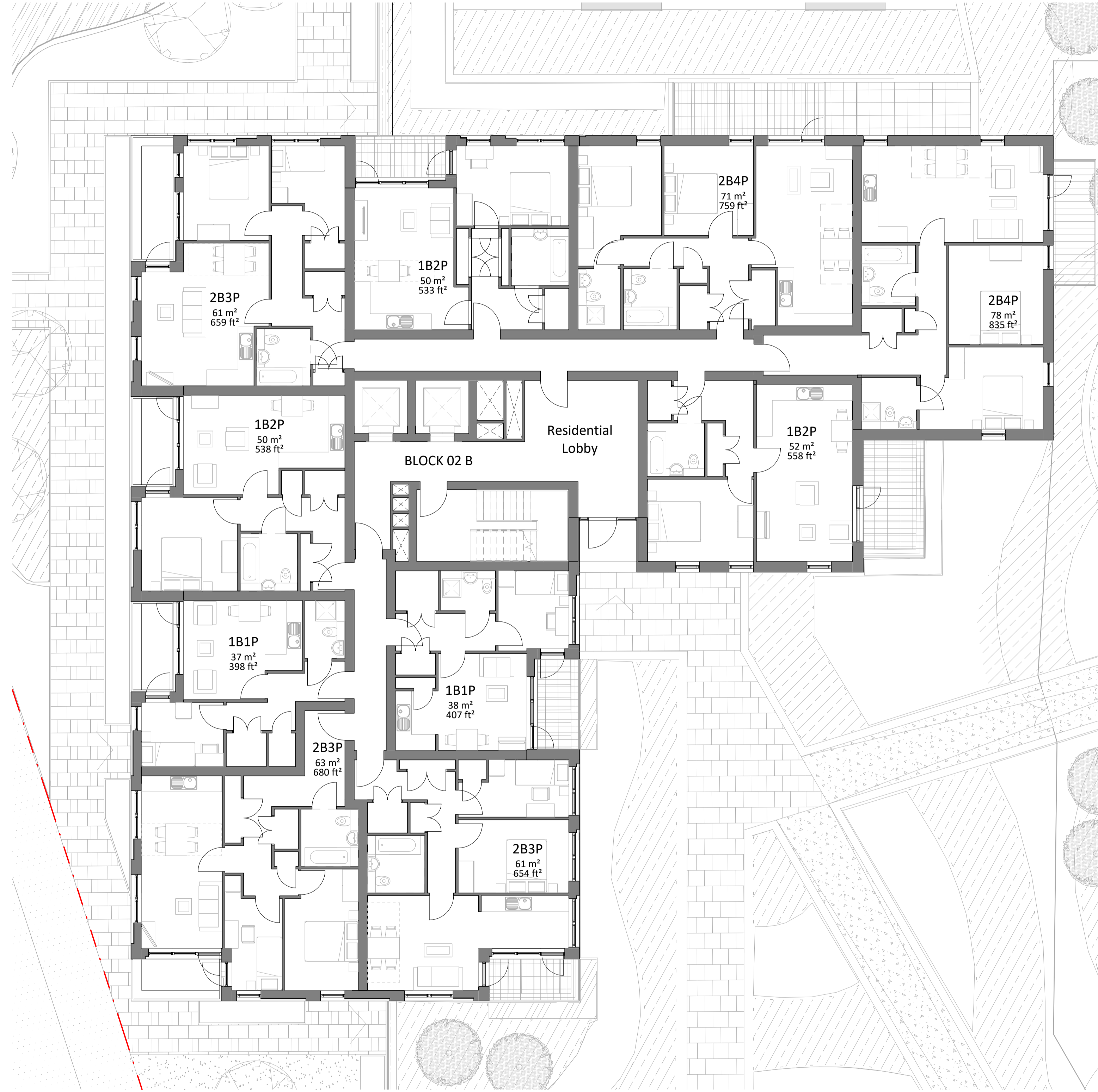
2 Block 02B - First Floor Plan 1 : 100 @A1
