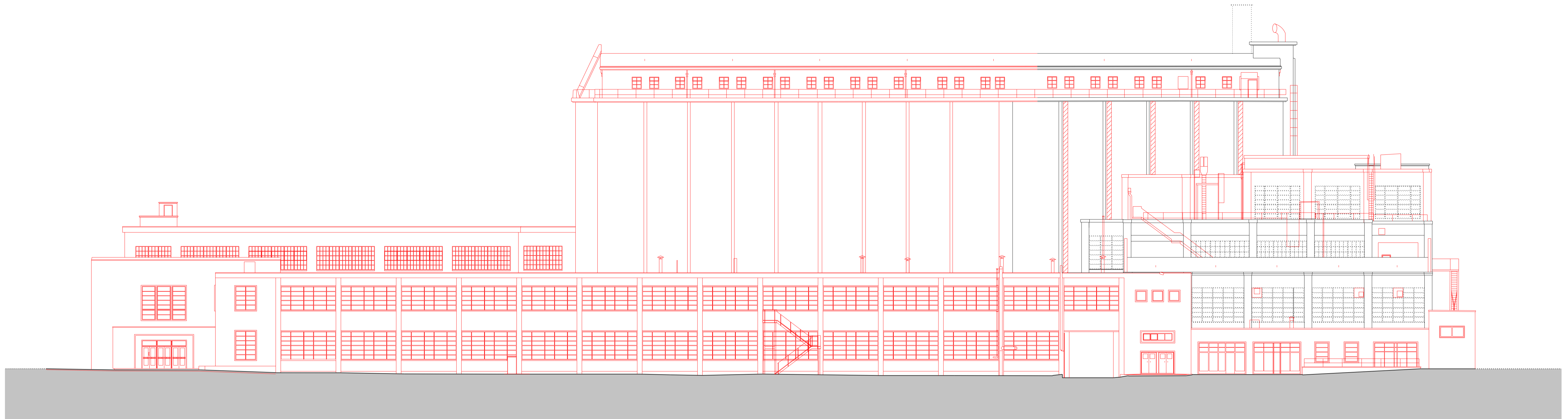
01. NORTH ELEVATION
