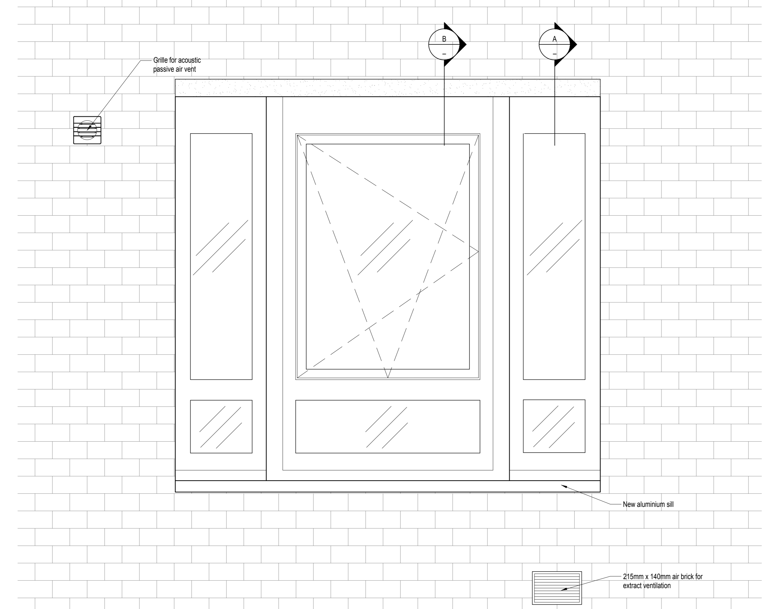
EXTERNAL ELEVATION EXTRACT SCALE: 1:10 @ A0
