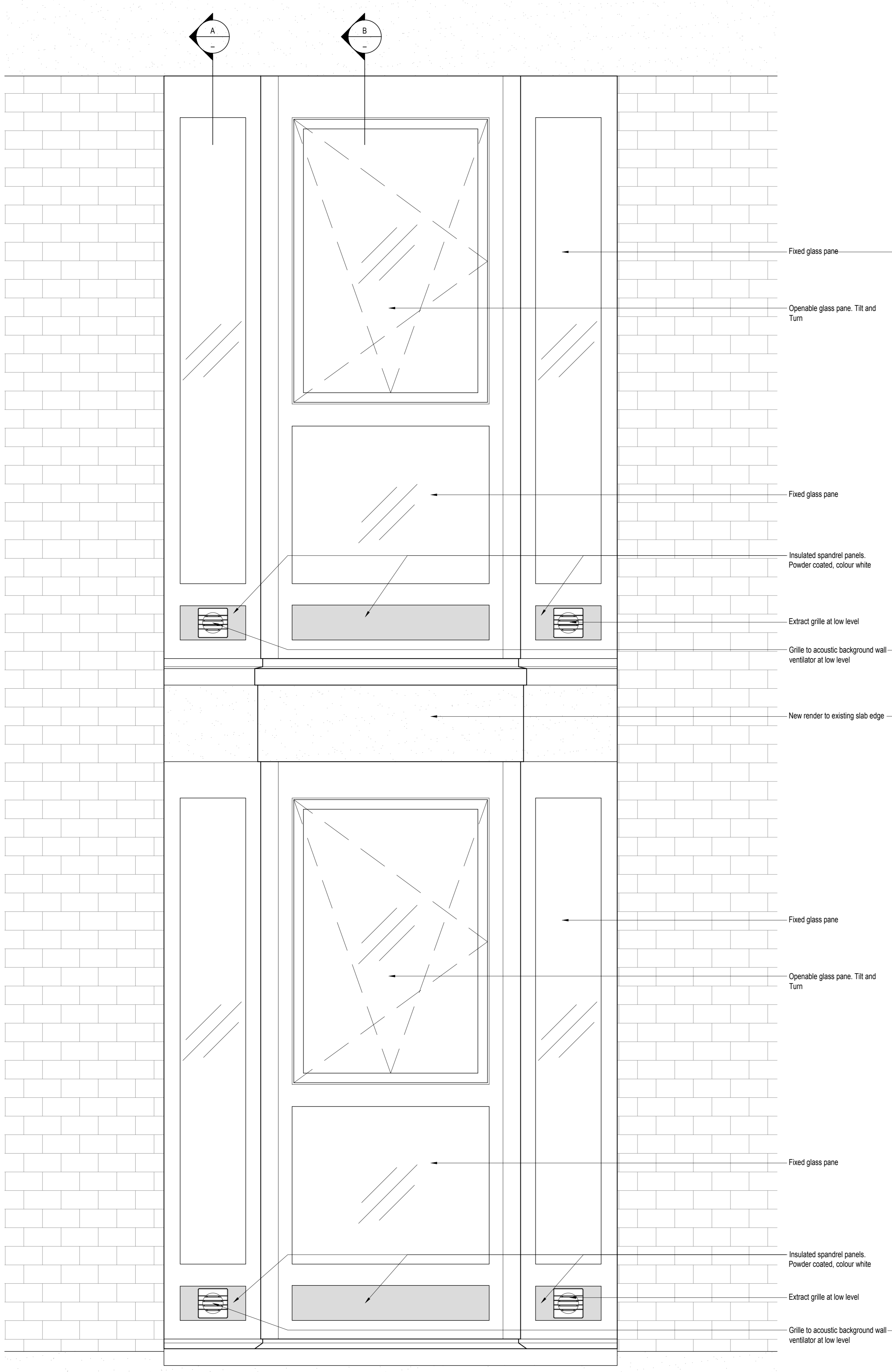
EXTERNAL ELEVATION EXTRACT SCALE: 1:10 @ A0
