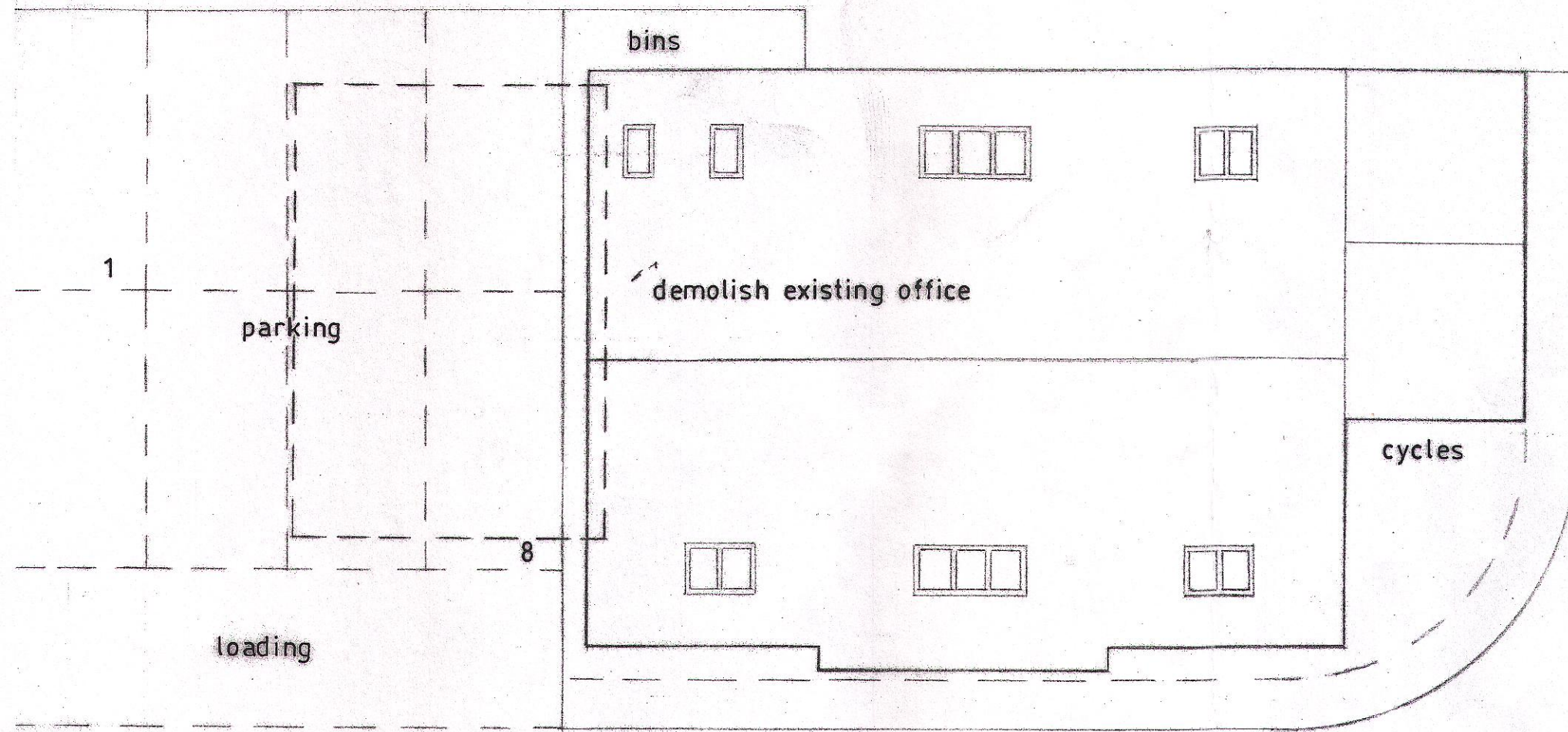
SITE/ROOF PLAN
