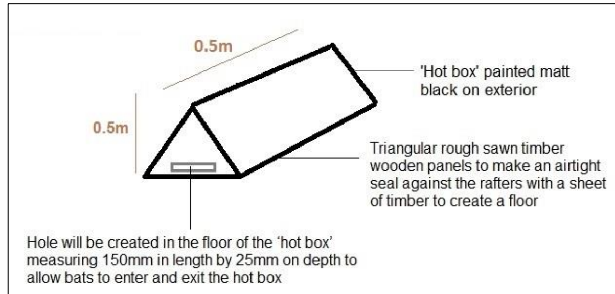
Figure 6 'Hot-box' design
