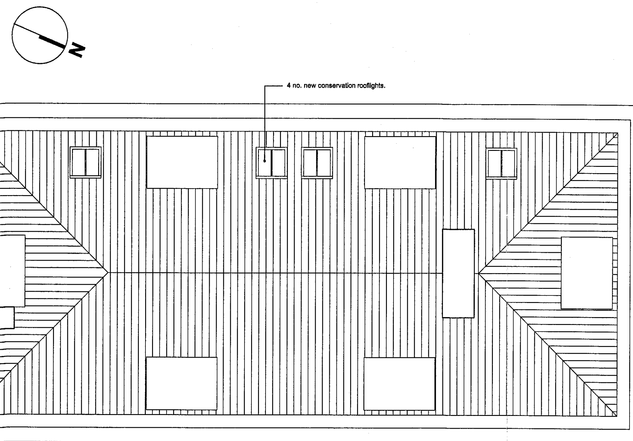
ROOF PLAN
