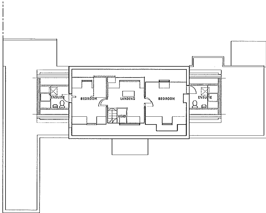
LOFT FLOOR PLAN
