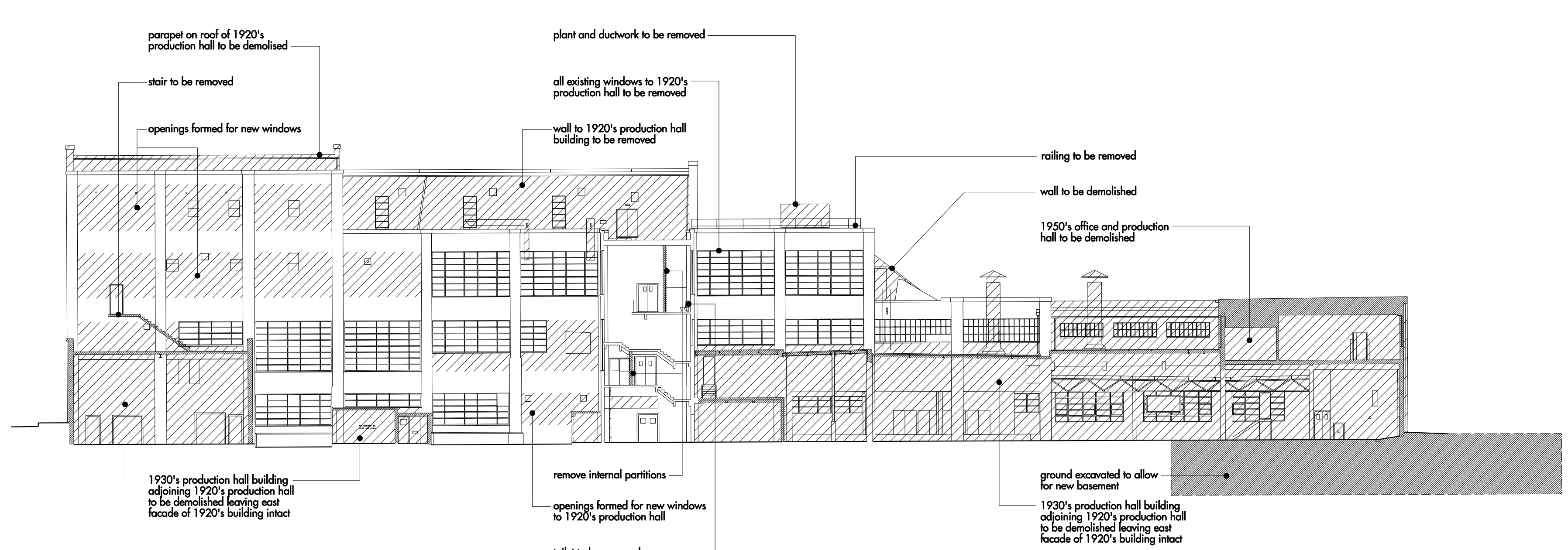
Section 03
