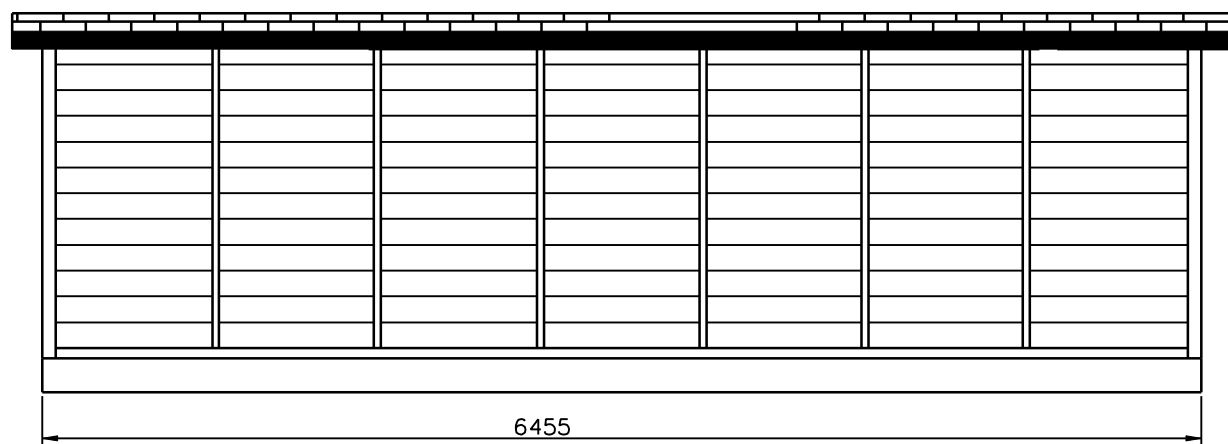
REAR ELEVATION B-B SCALE 1:50
